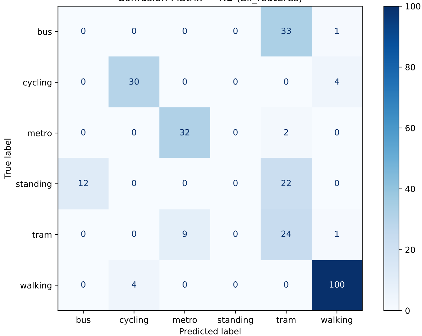
Confusion Matrix — NB (all_features)
