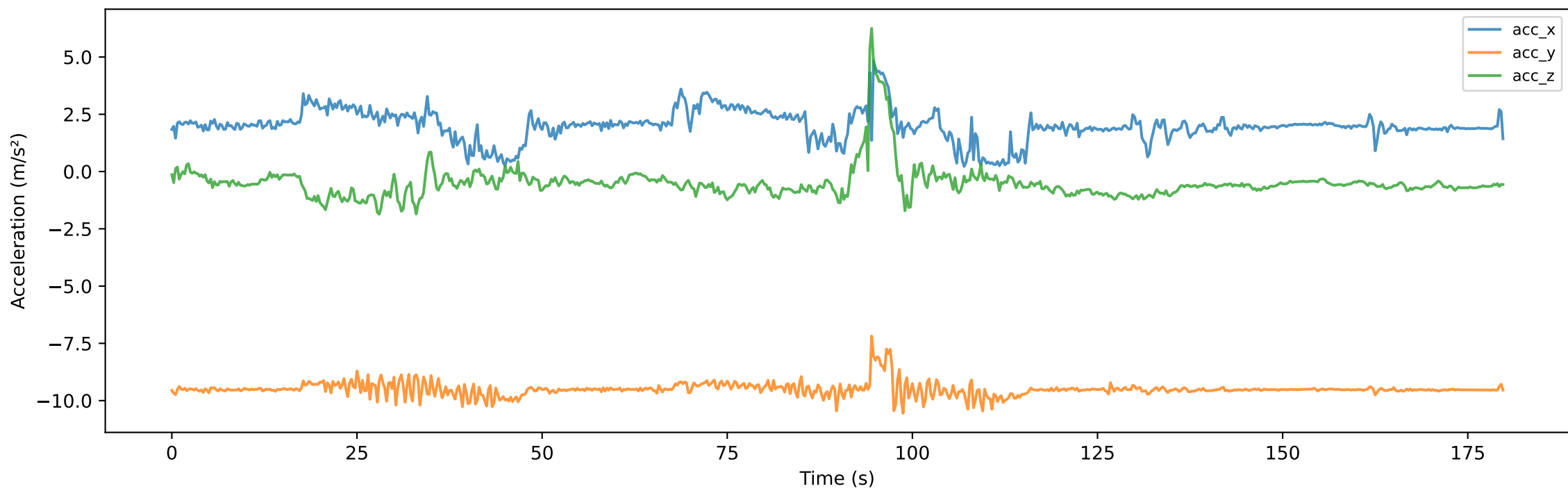
Linear Accelerometer — tram
