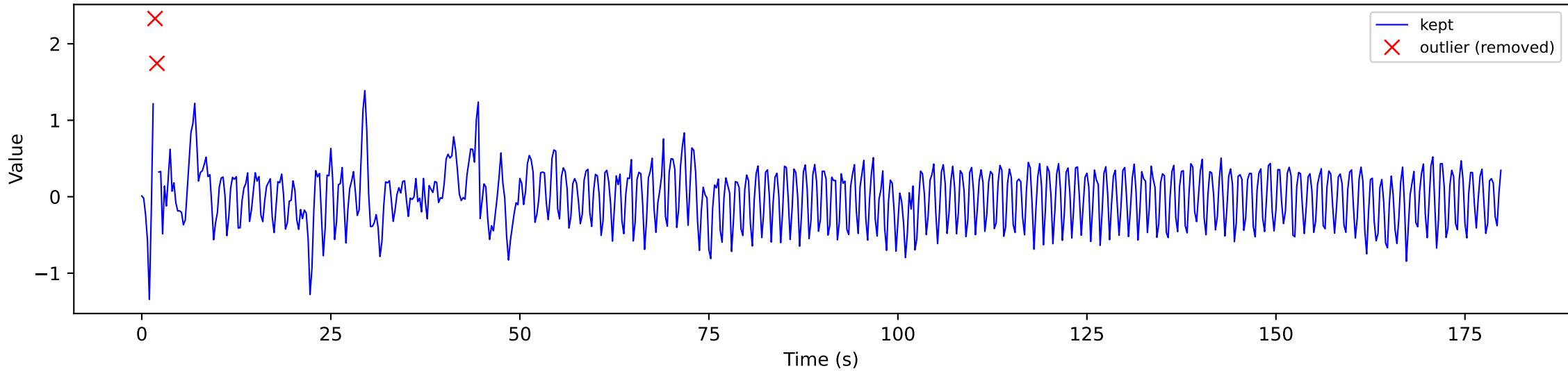
gyr_z — after Chauvenet outlier removal (C=2)
