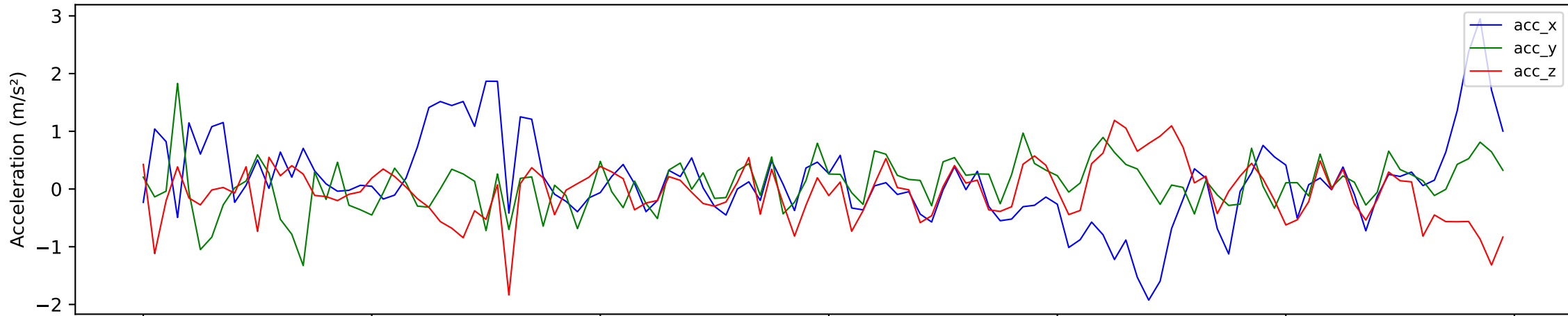
Accelerometer — after low-pass filter (cutoff=1.5 Hz)
