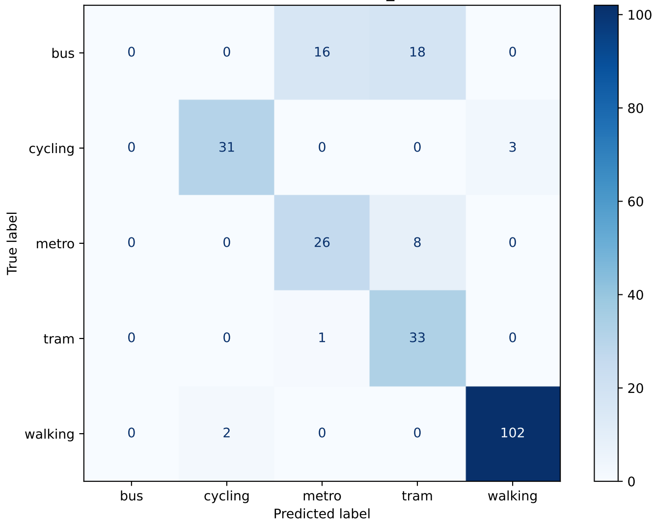
Confusion Matrix — RF (all_features)
