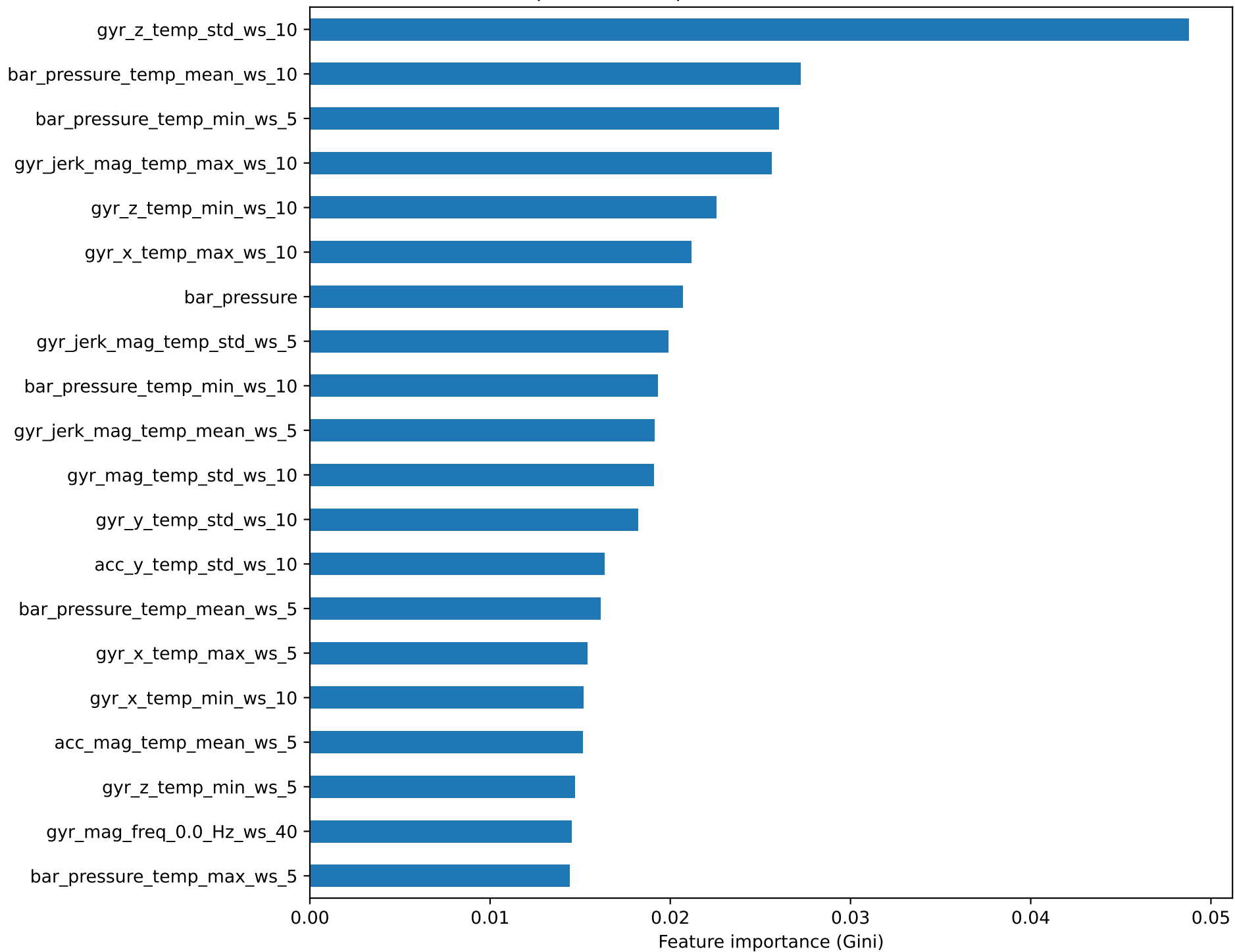
Top 20 most important features (Random Forest)
