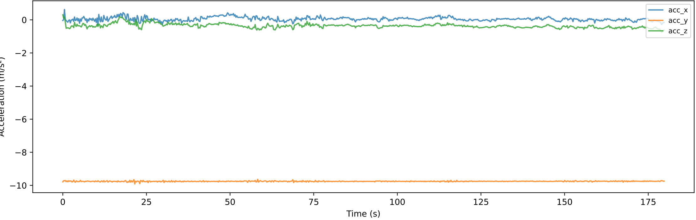
Linear Accelerometer — bus
