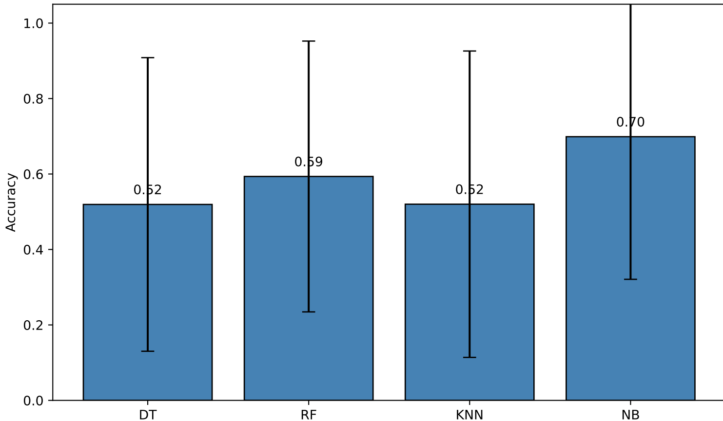
Leave-One-Session-Out CV — Mean Accuracy ( \pm std)
