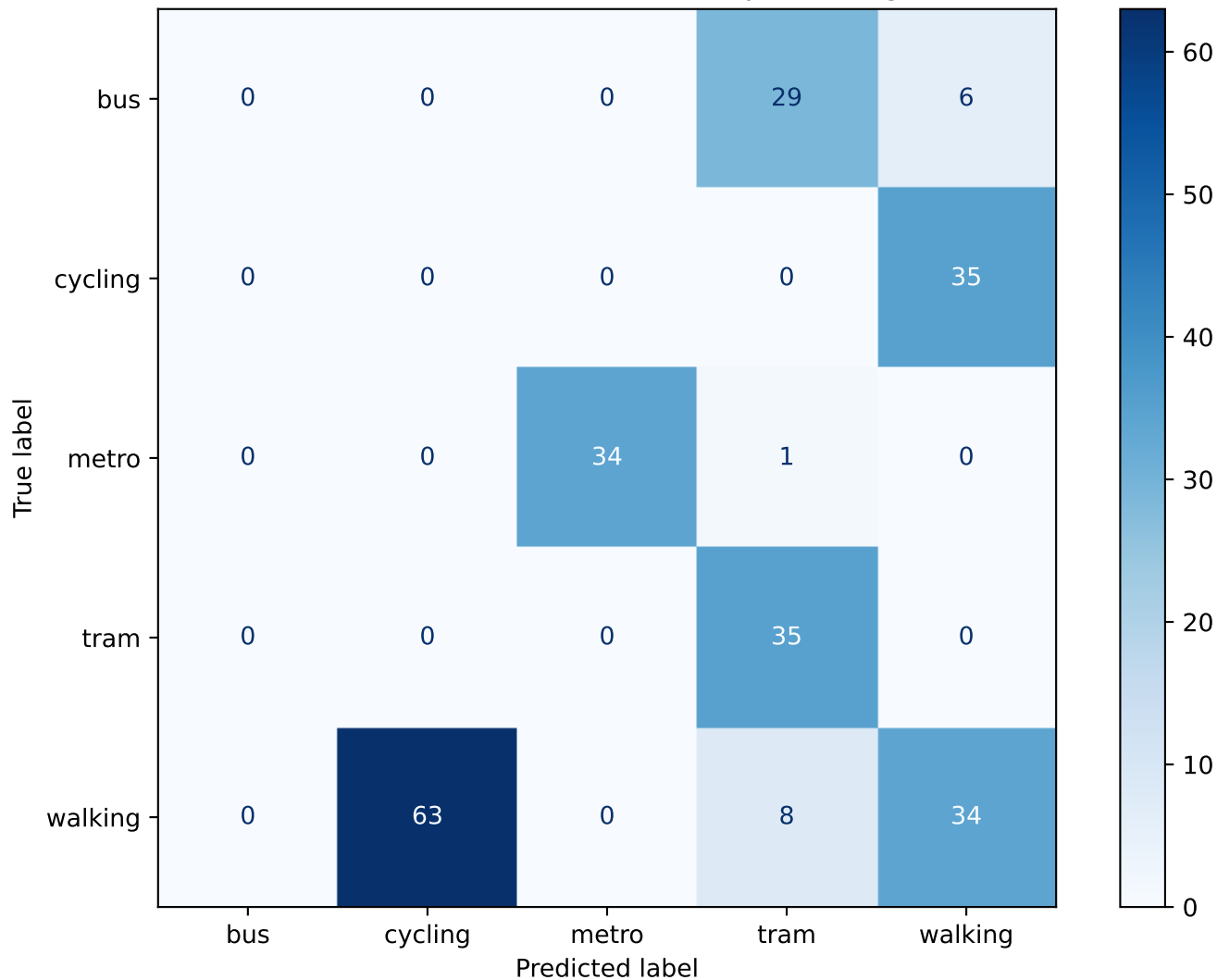
Confusion Matrix — CNN (Deep Learning)
