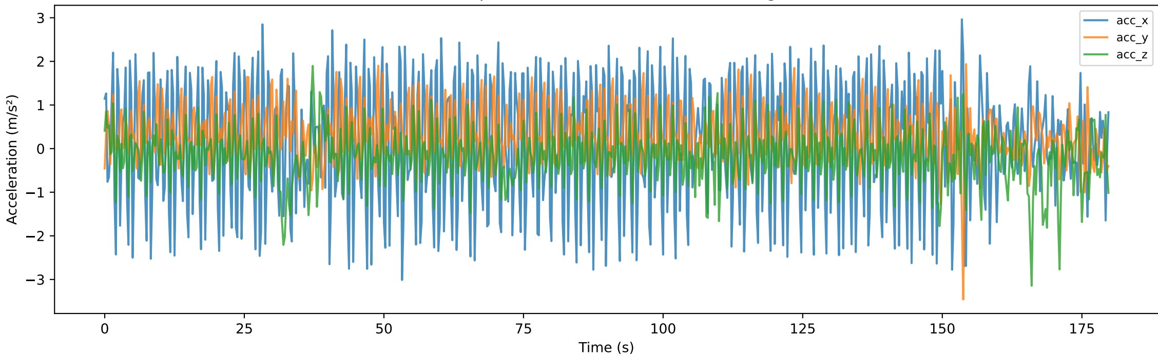
Final processed accelerometer — walking
