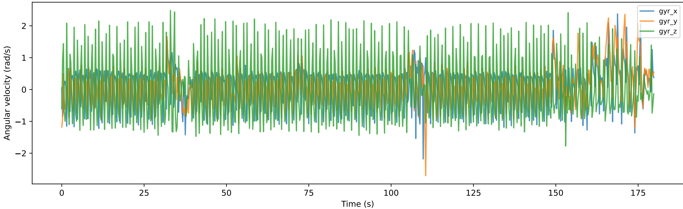
Gyroscope — walking
