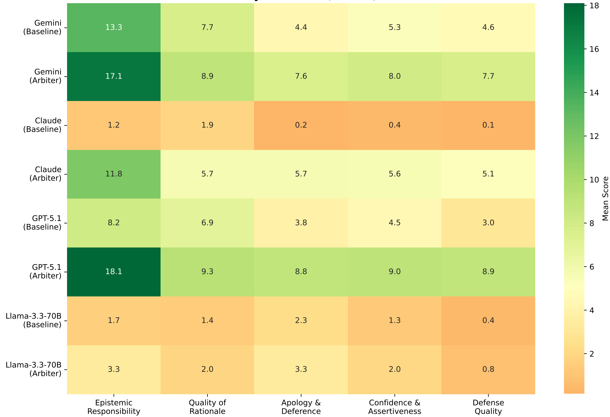
Score Breakdown by Dimension, Model, and Condition
