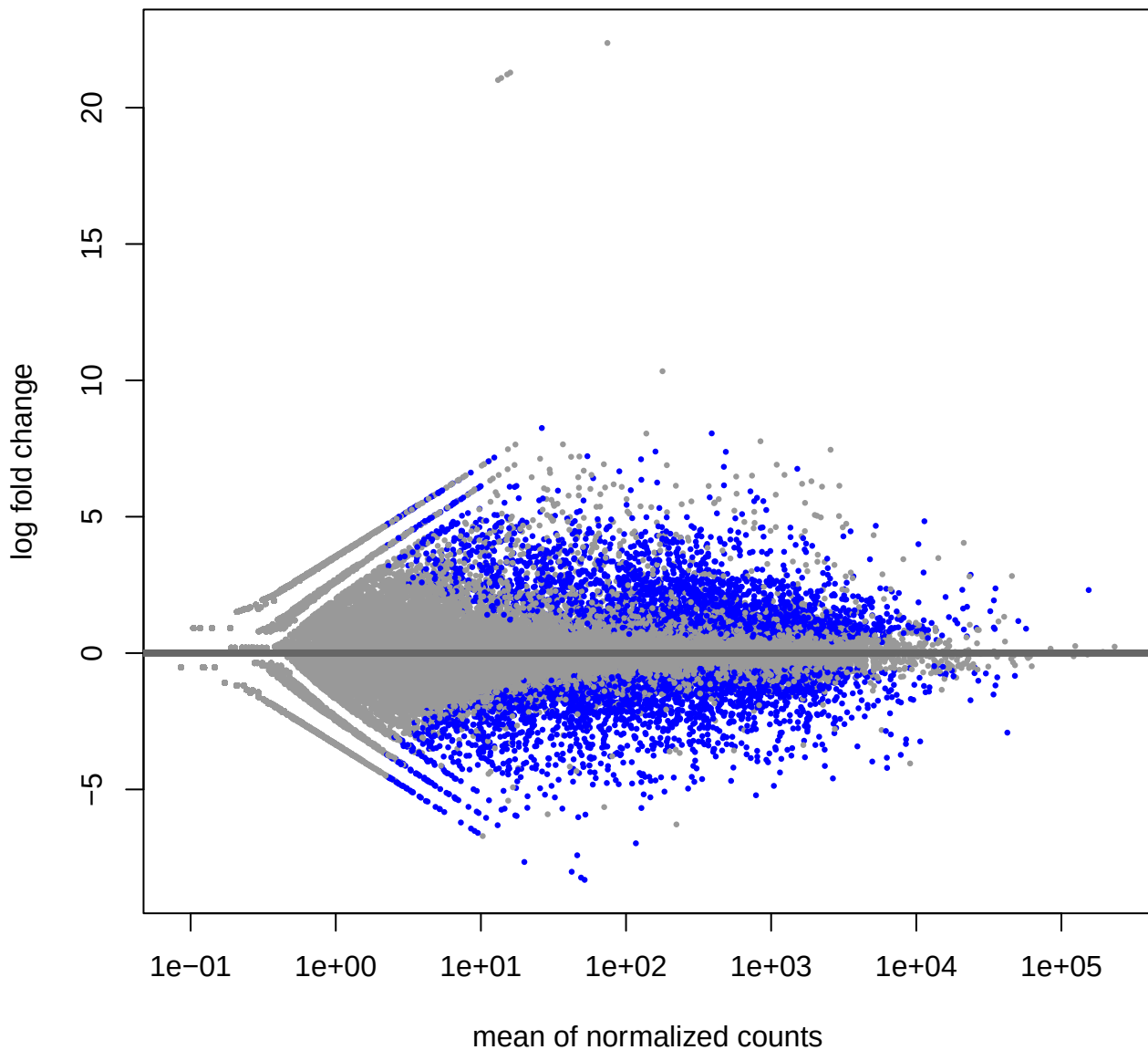
MA-plot for condition: TNBCXTumor vs Normal
