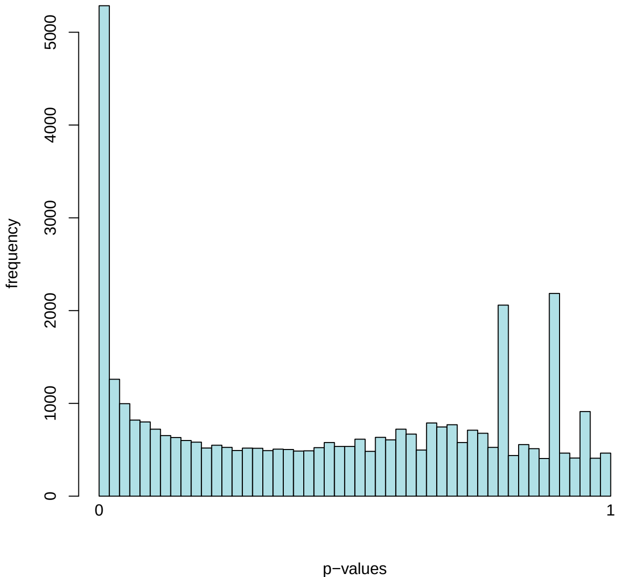
Histogram of p-values for condition: TNBCXTumor vs Normal
