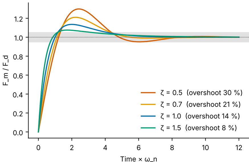
Normalised force step response (computed from transfer function)
