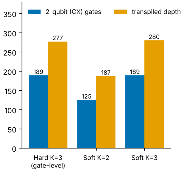
(b) Transpiled cost, opt. level 1
