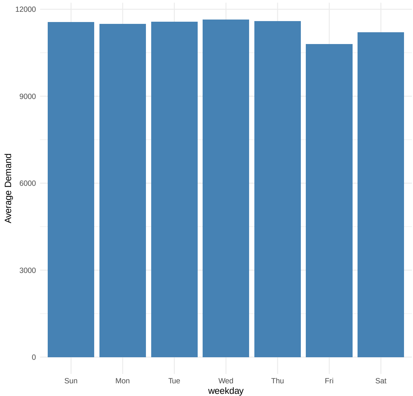
Day of Week Demand
