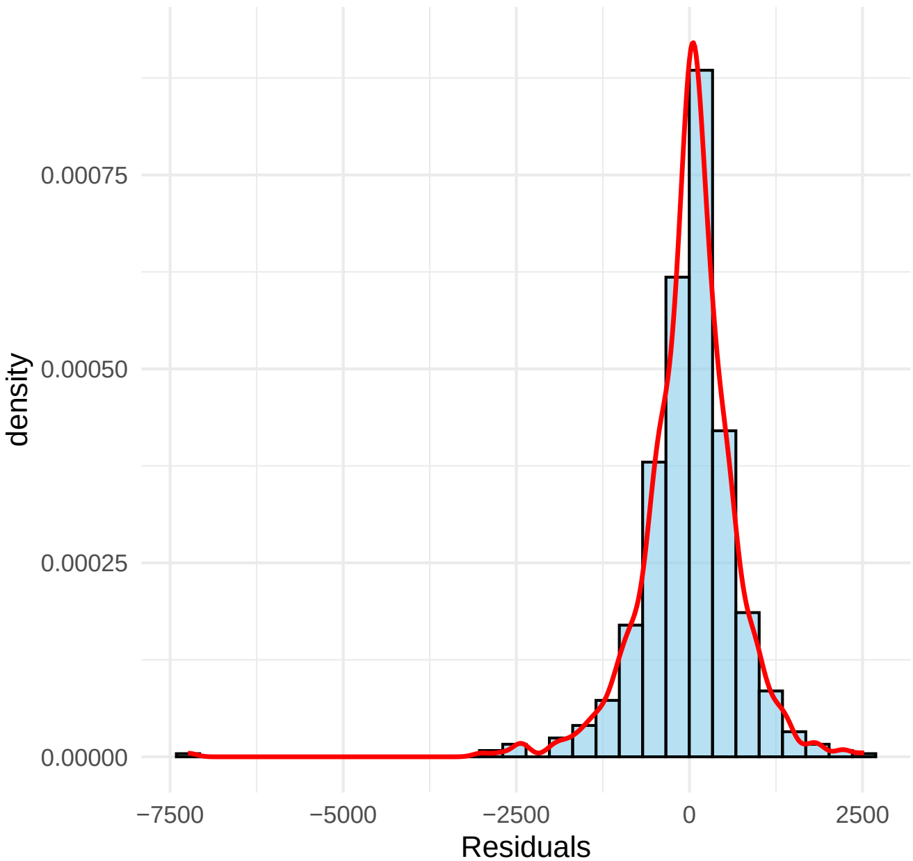
Histogram of SARIMA Residuals
