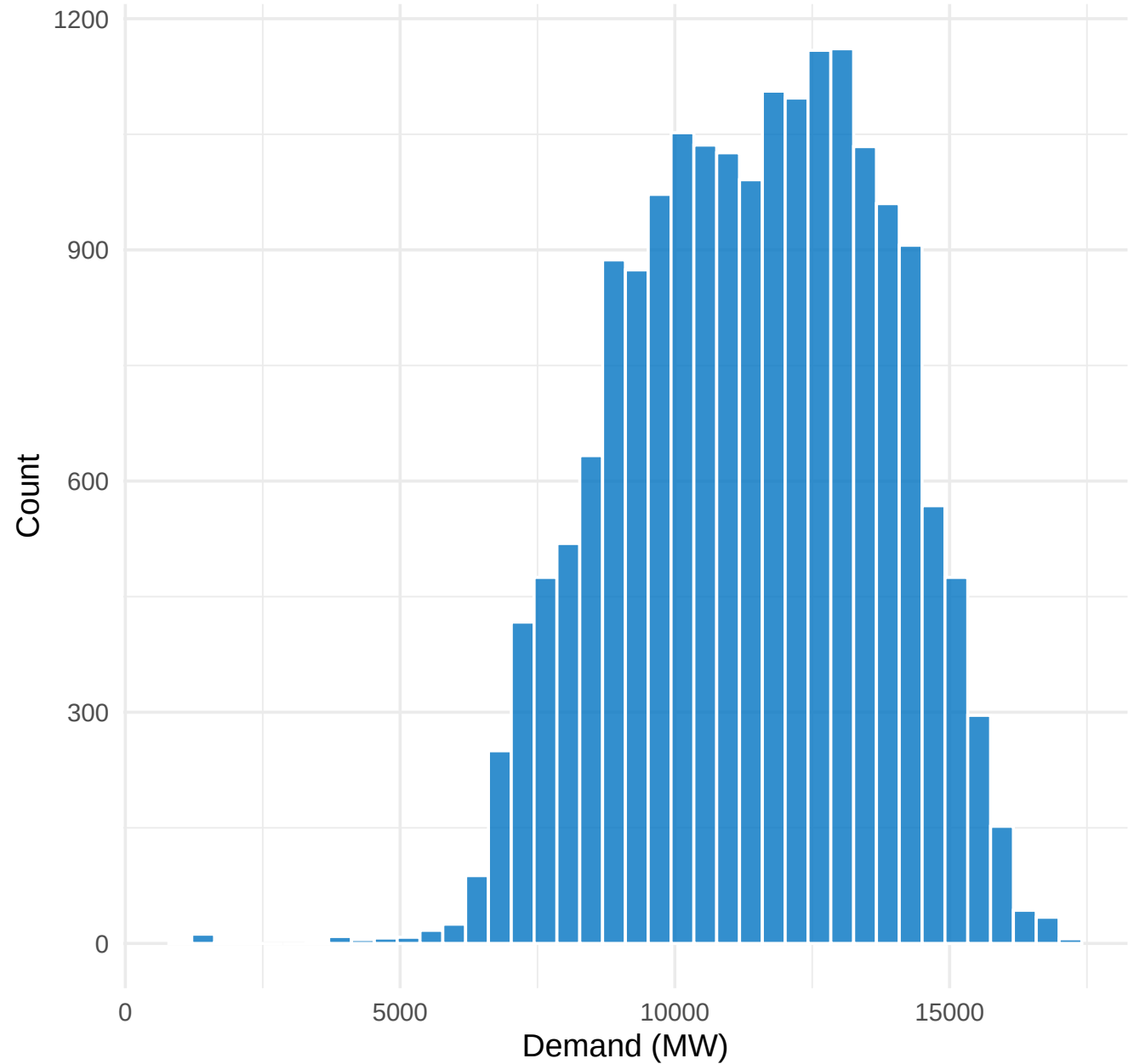
Distribution of Electricity Demand (MW)
