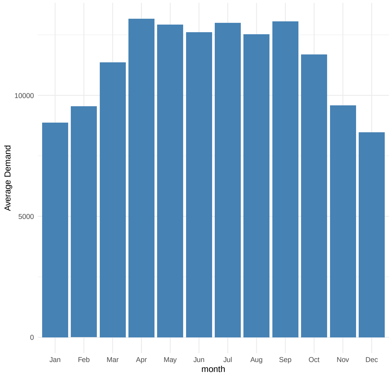
Monthly Demand Variation
