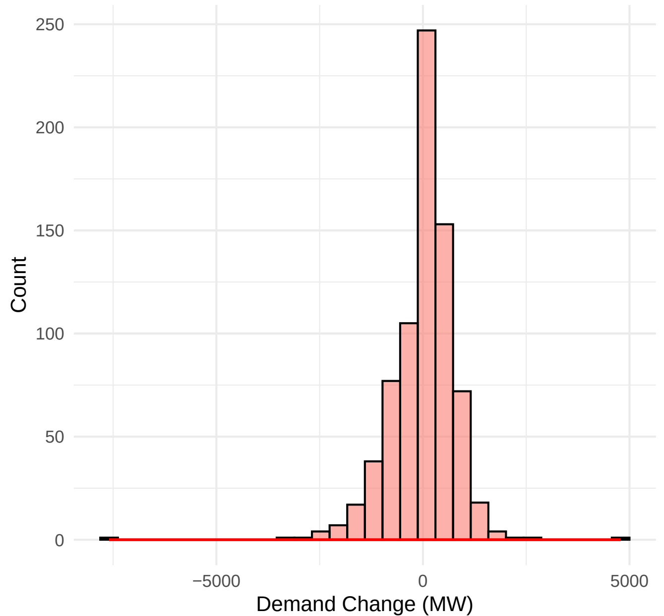
Distribution of Daily Demand Changes
