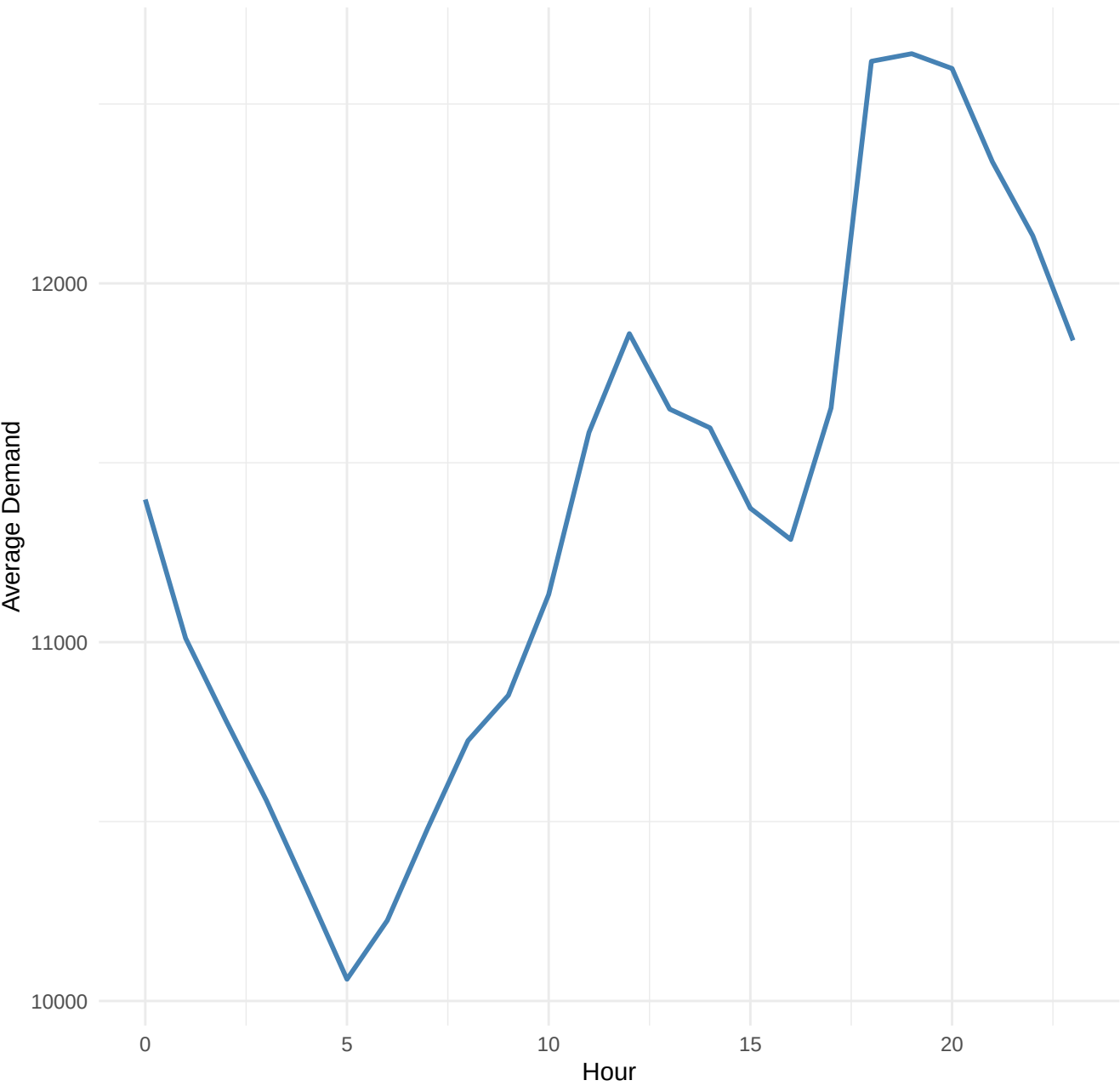
Hourly Demand Pattern
