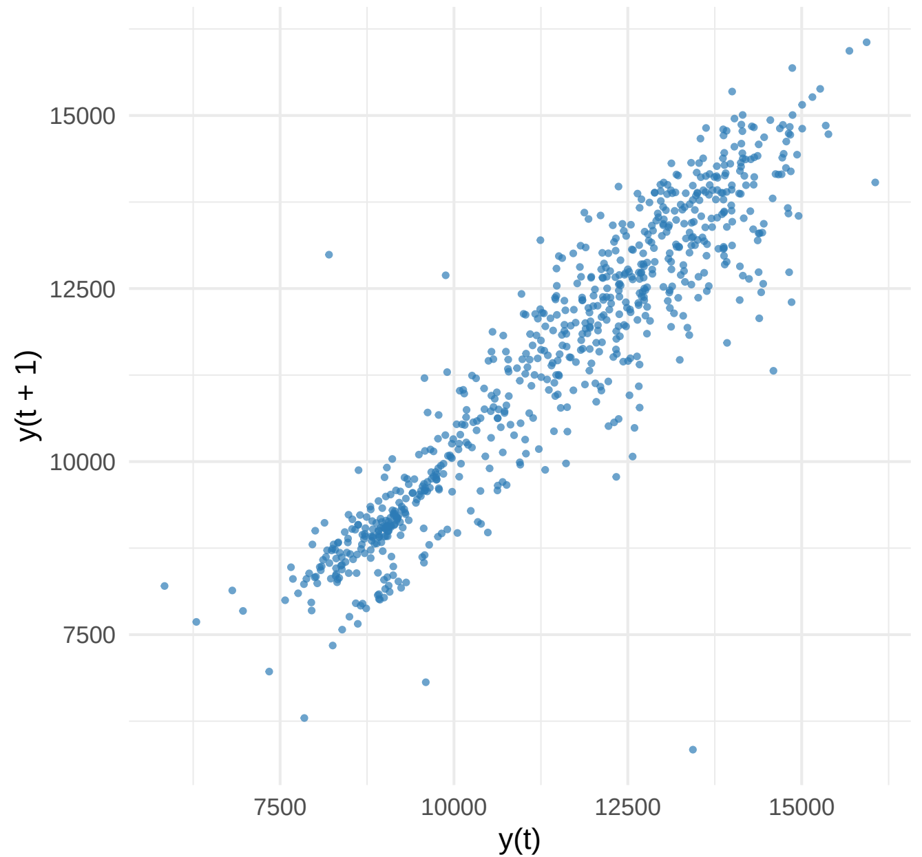
Lag Plot – Daily Electricity Demand
