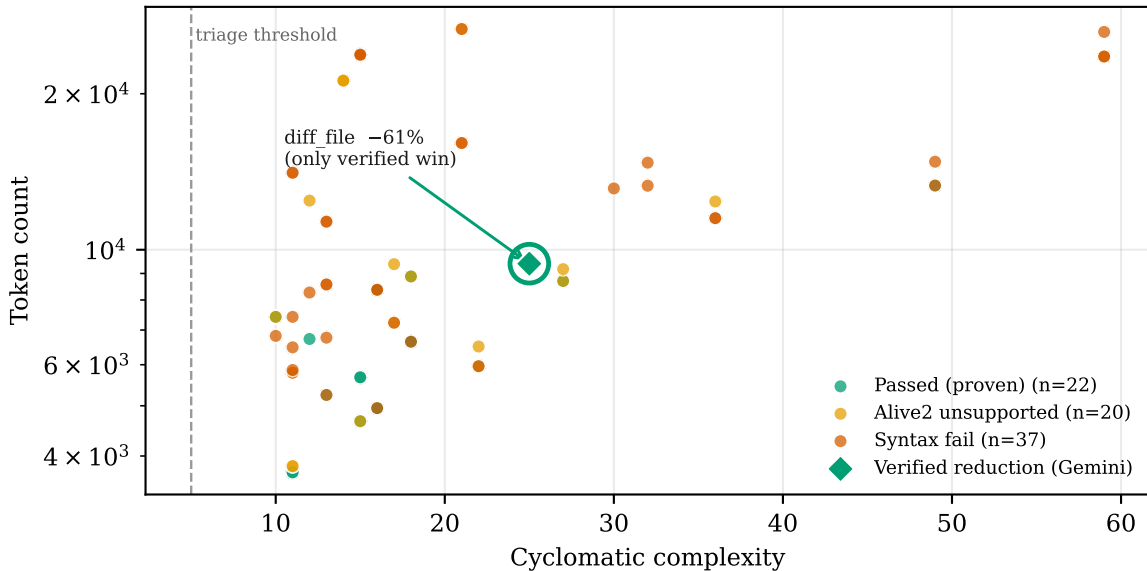
The capability cliff: verified optimisation is a point, not a region
