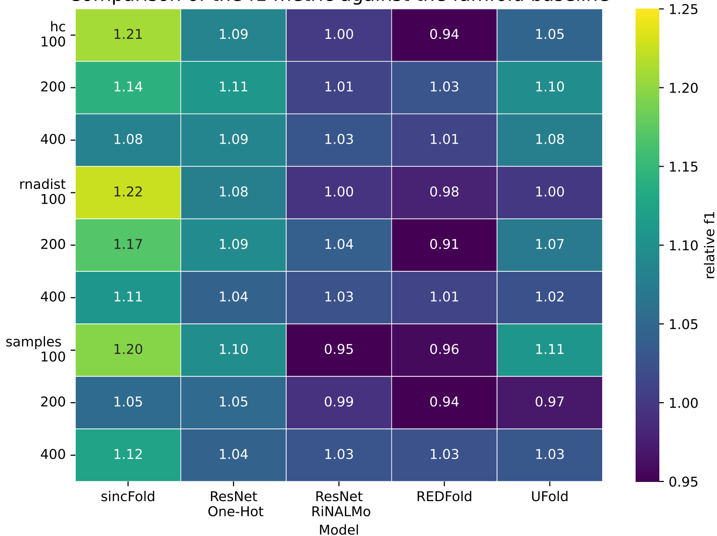
Comparison of the f1 metric against the famfold baseline
