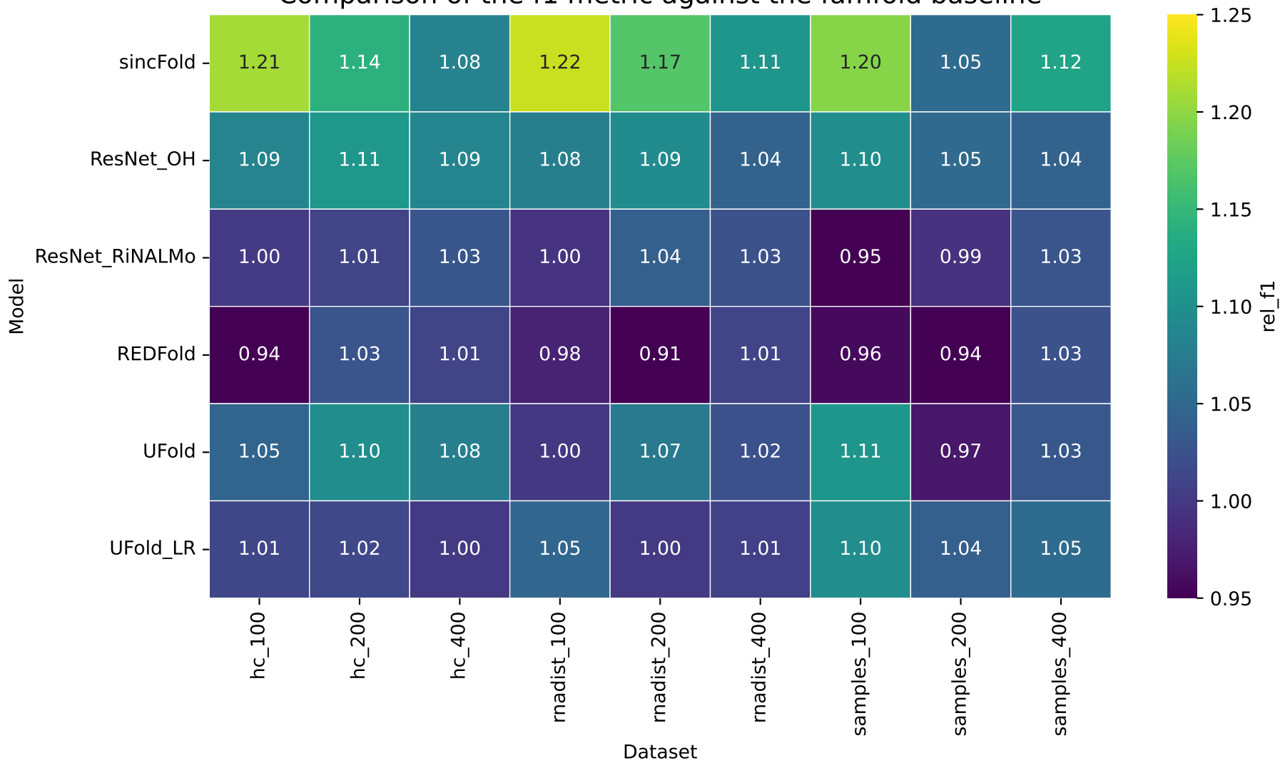
Comparison of the f1 metric against the famfold baseline
