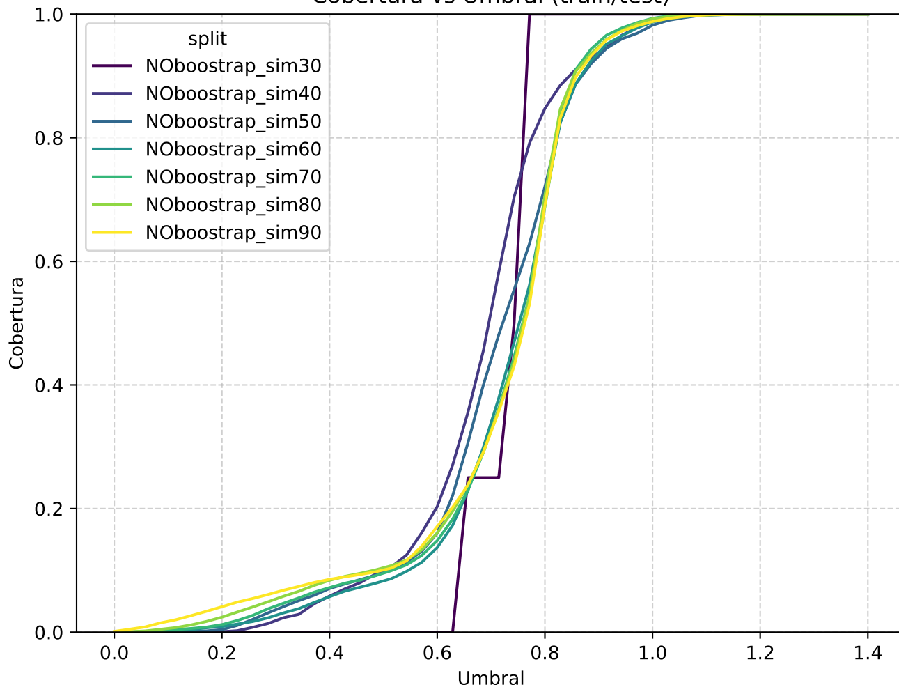
Cobertura vs Umbral (train/test)
