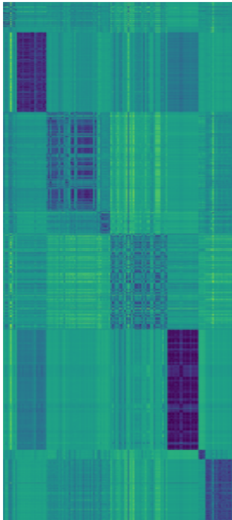
NObootstrap_sim90
