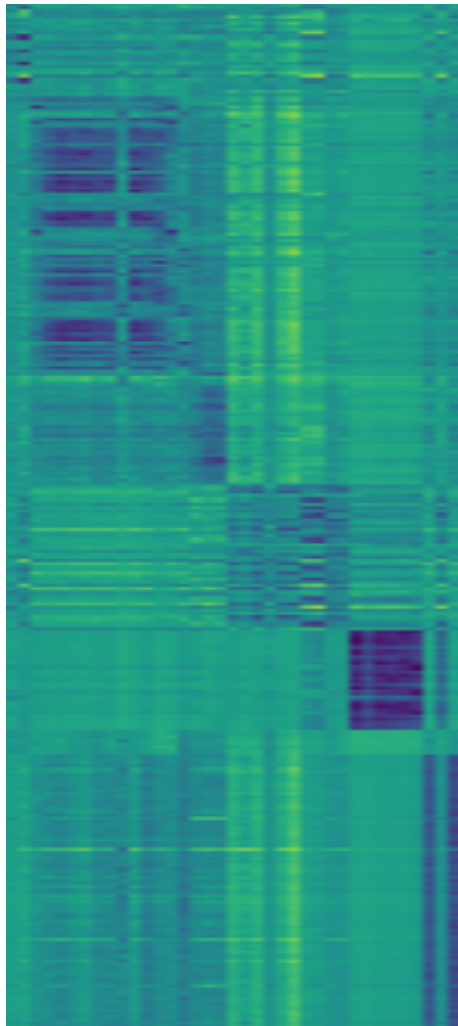
NObootstrap_sim60
