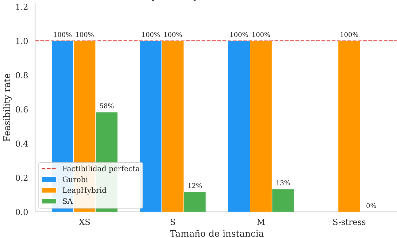
Feasibility rate by solver and instance size
