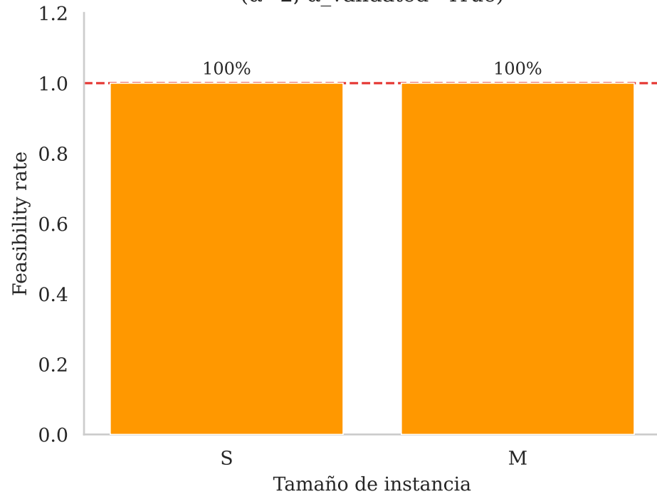
LeapHybrid validation feasibility ( \alpha=2 , \alpha\_validated=True )
