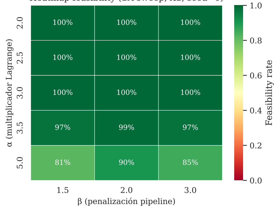
Heatmap feasibility (SA sweep, XS, seed=0)
