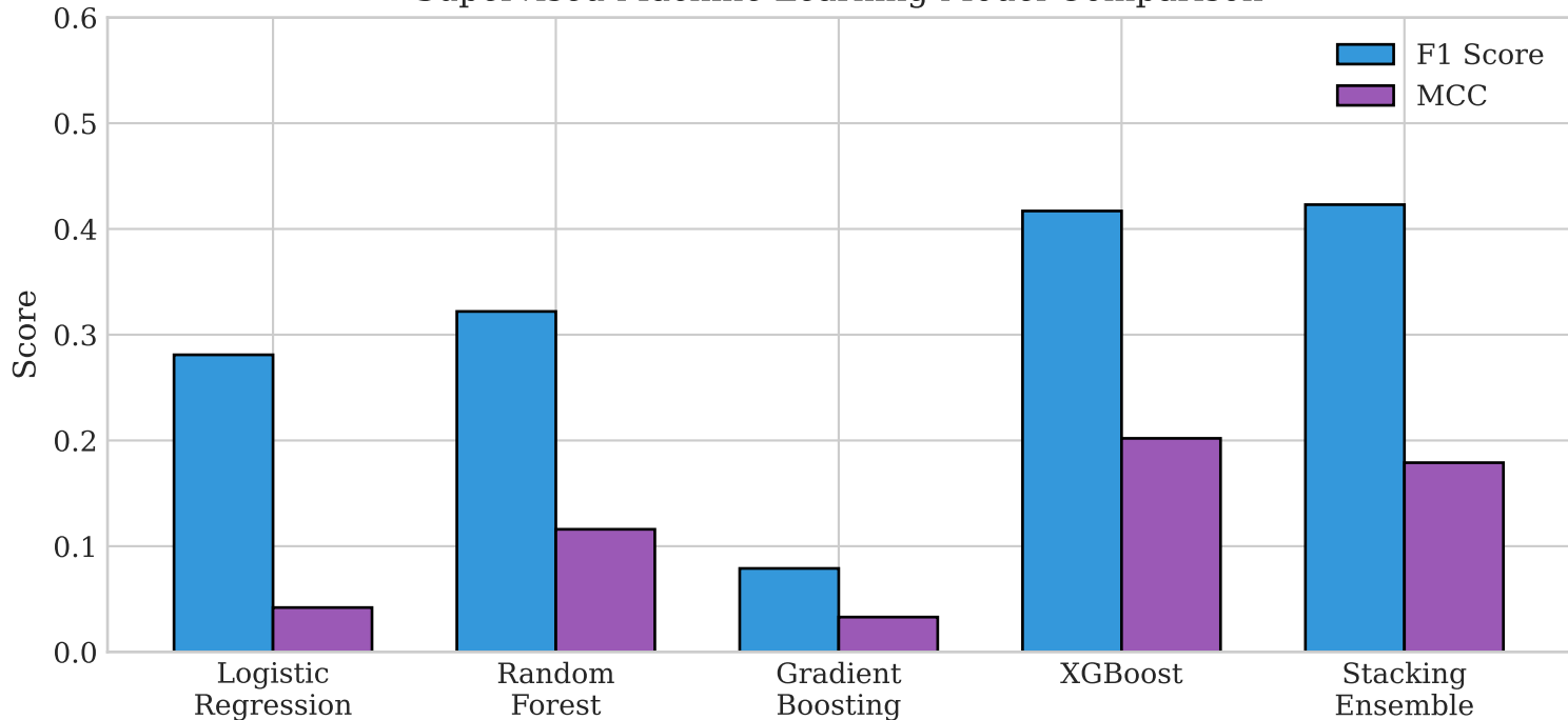
Supervised Machine Learning Model Comparison
