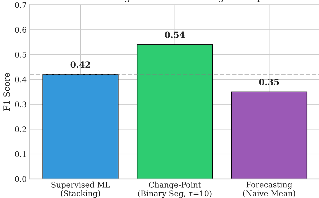
Real-World Bug Prediction: Paradigm Comparison
