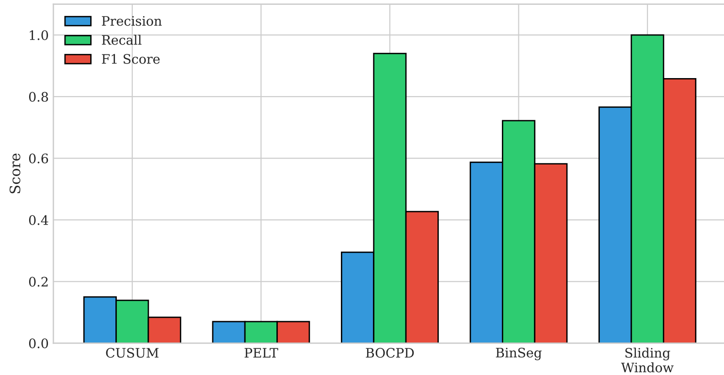
Change-Point Detection Algorithm Comparison
