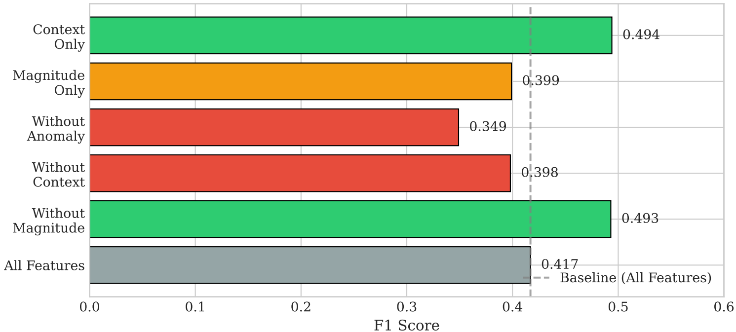
Feature Ablation Study: Impact of Feature Groups
