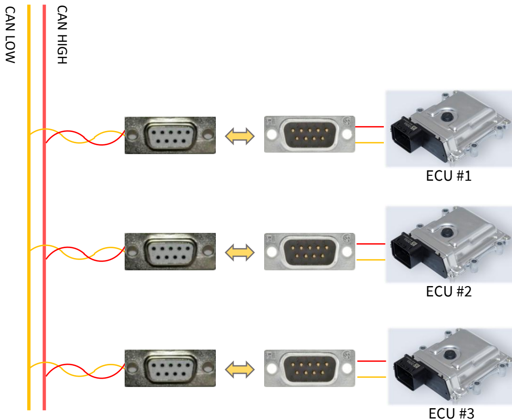
CAN connection
