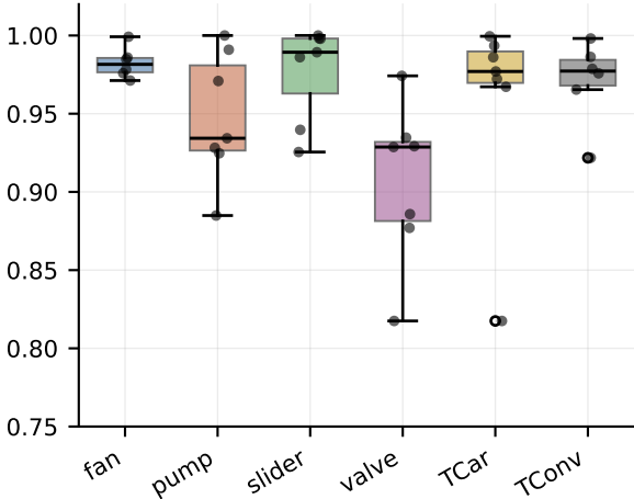
File-level ROC-AUC
