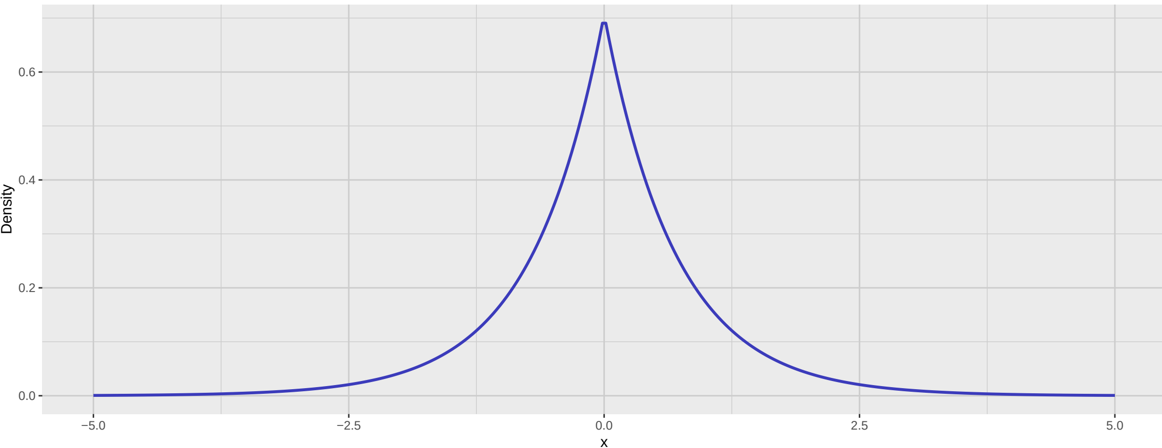
Laplace Distribution PDF (mean = 0, sd = 1)
