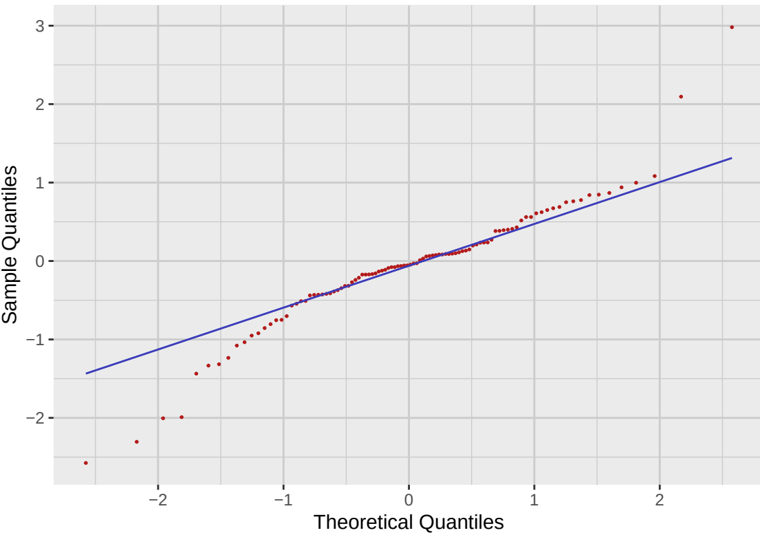
QQ Plot
