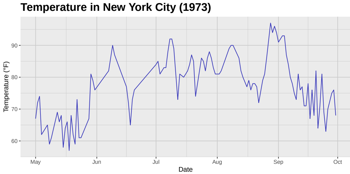
Figure 3: Temperature in New York City from May to September 1973
