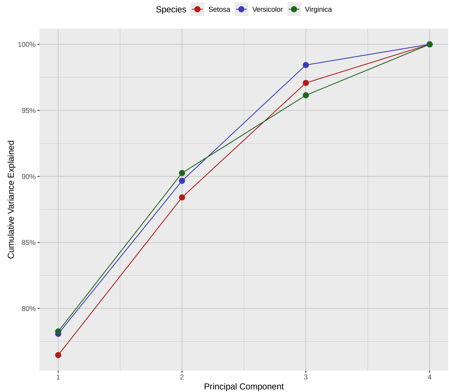
Cumulative Variance Explained by Principal Components
