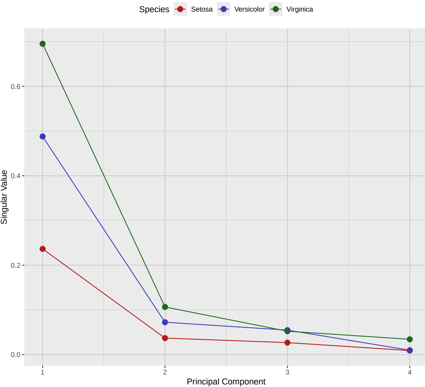
Scree Plot of Iris Dataset
