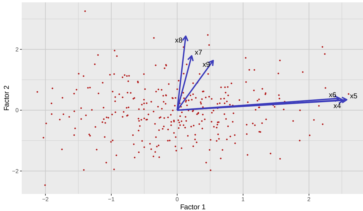
Figure 8.1: Factor Analysis Biplot of the Holzinger Swineford 1939 Dataset
