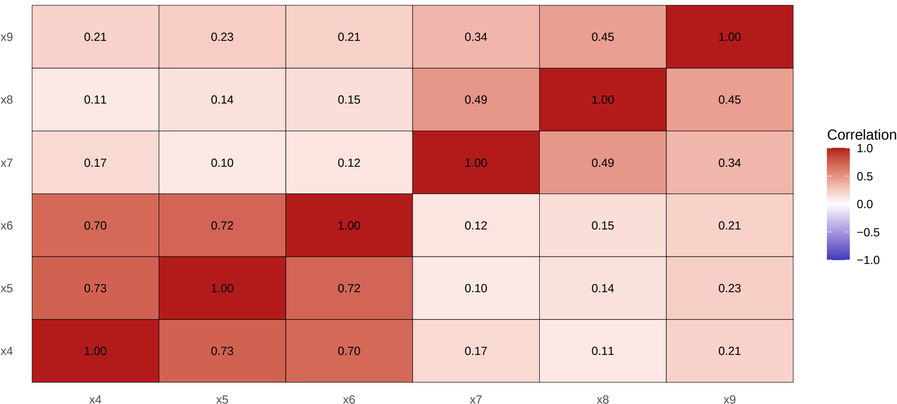
Correlation heatmap for tests x4-x9
