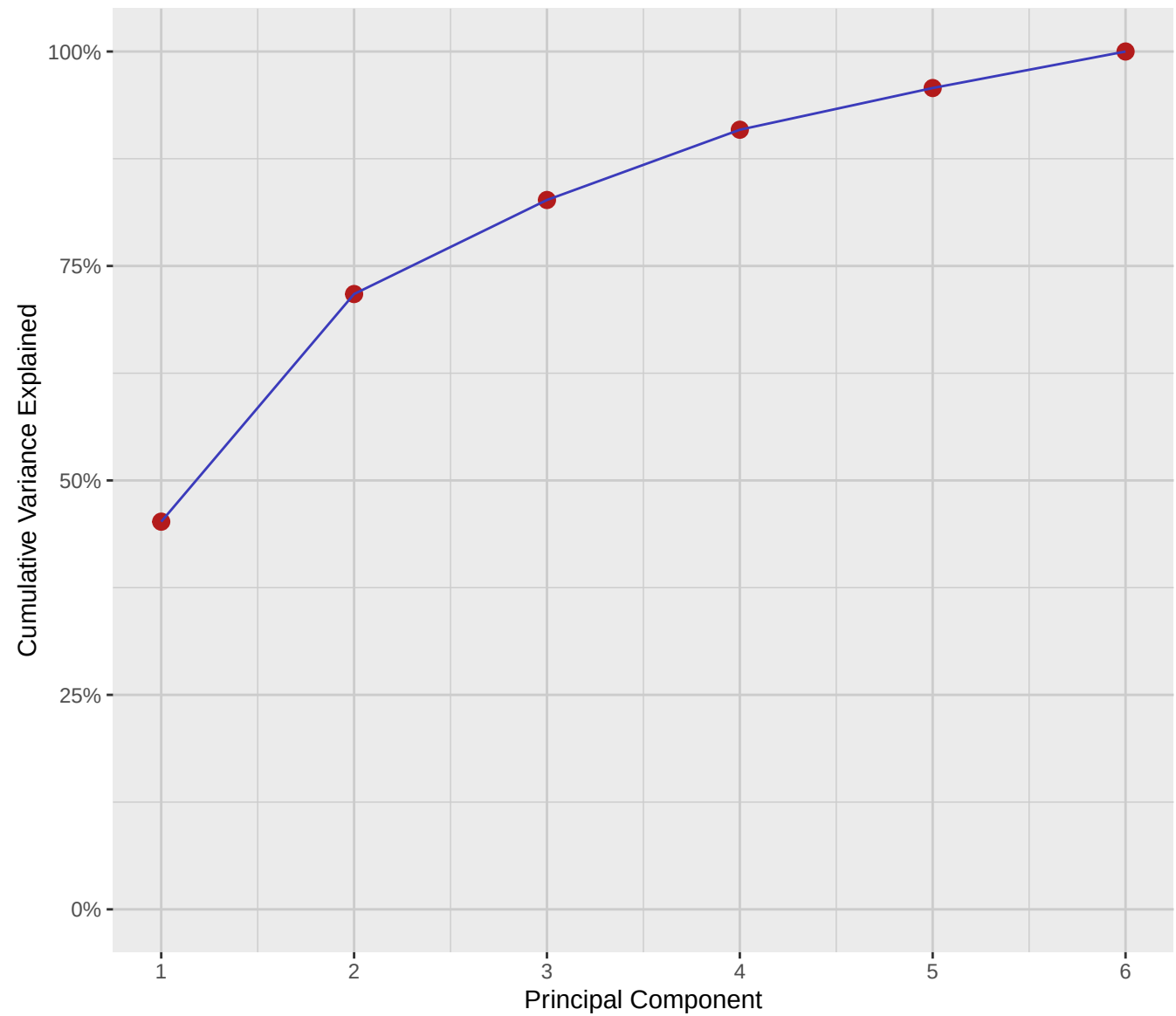
Cumulative Variance Plot
