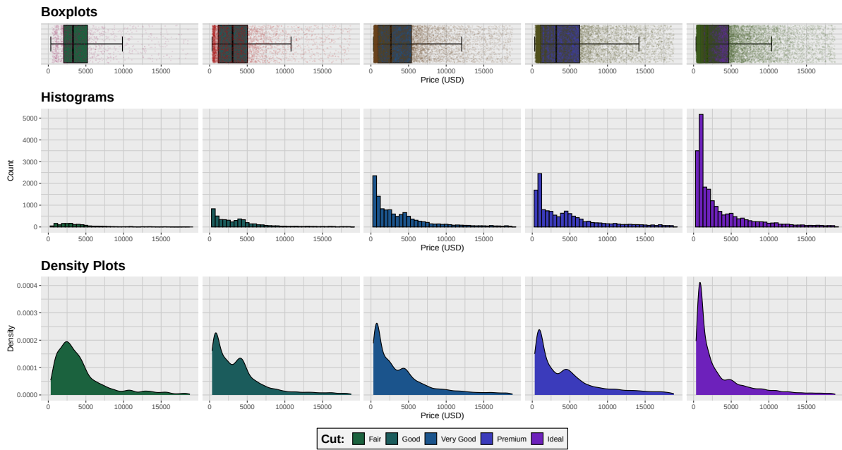
Figure 9: Plot showing the boxplots, histograms and density plots corresponding to the price of diamonds by cut
