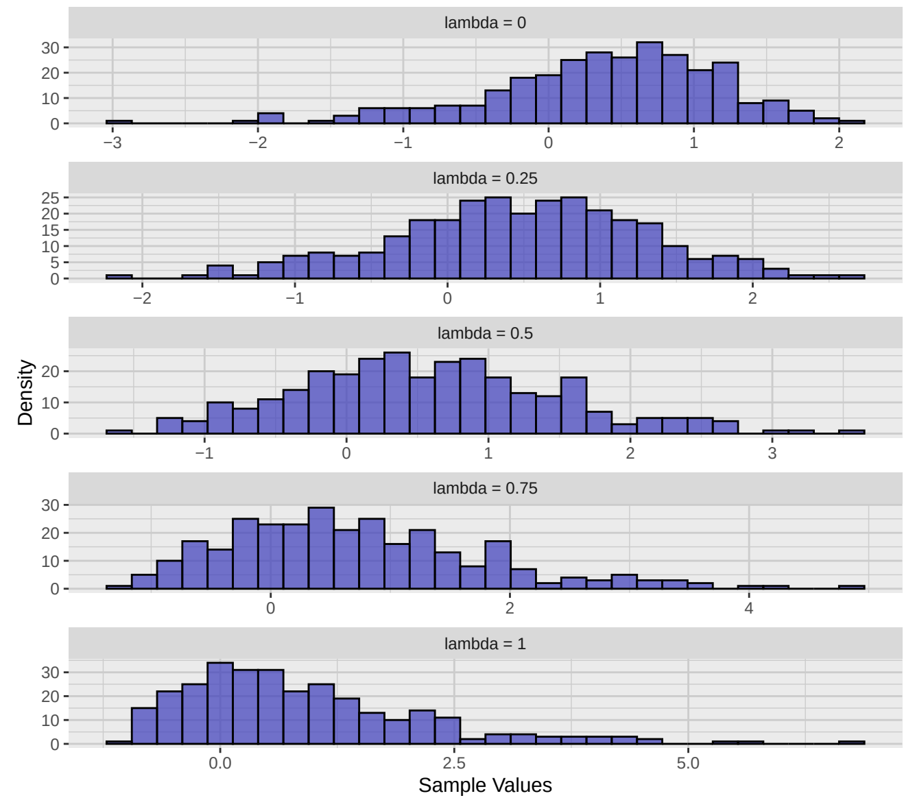
Histograms
