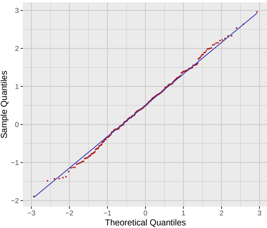
QQ Plot
