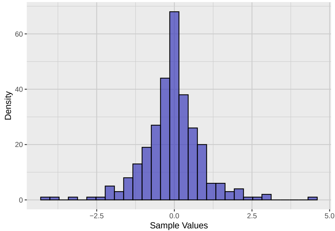
Histogram
