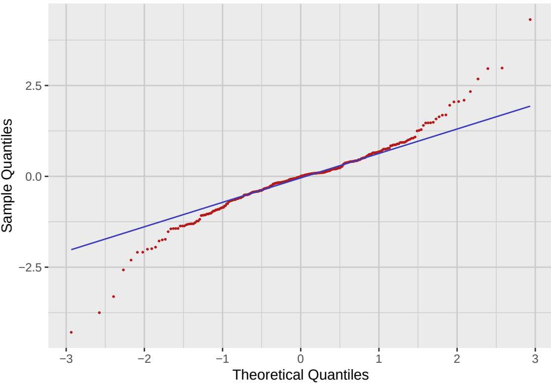
QQ Plot
