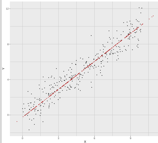
First Principal Component Projection
