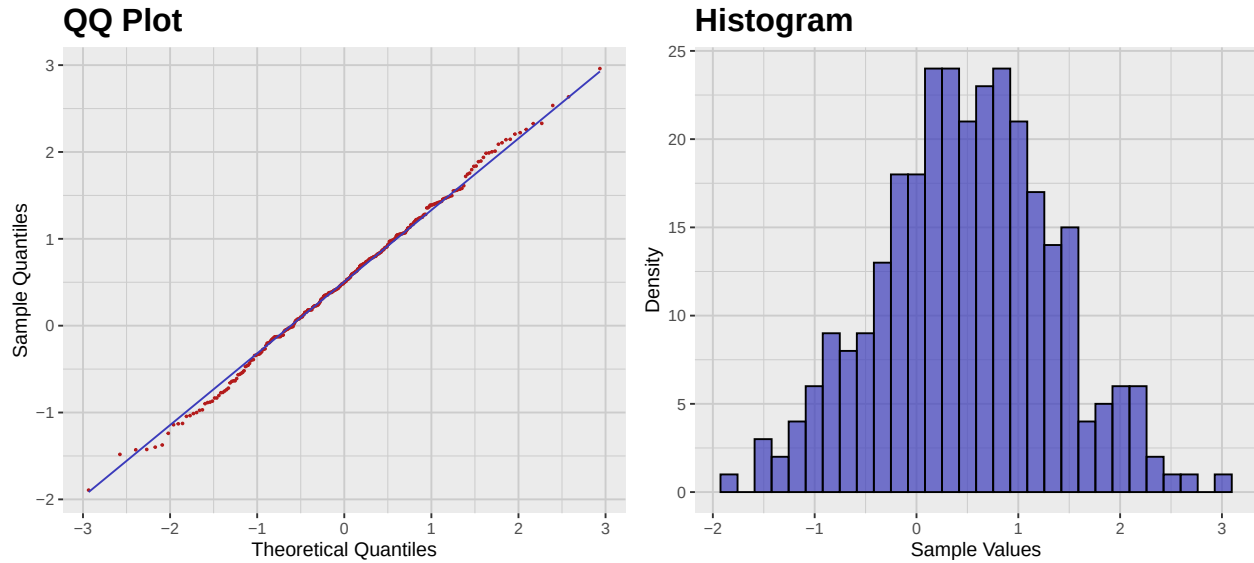
Figure 3.2: QQ plot and histogram of the Optimal Gamma Distribution Transformation. Notice how both plots show a much better fit to the normal distribution compared to the original gamma sample.
