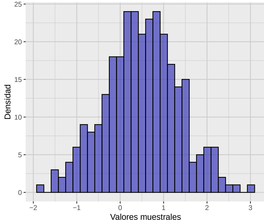
Histograma
