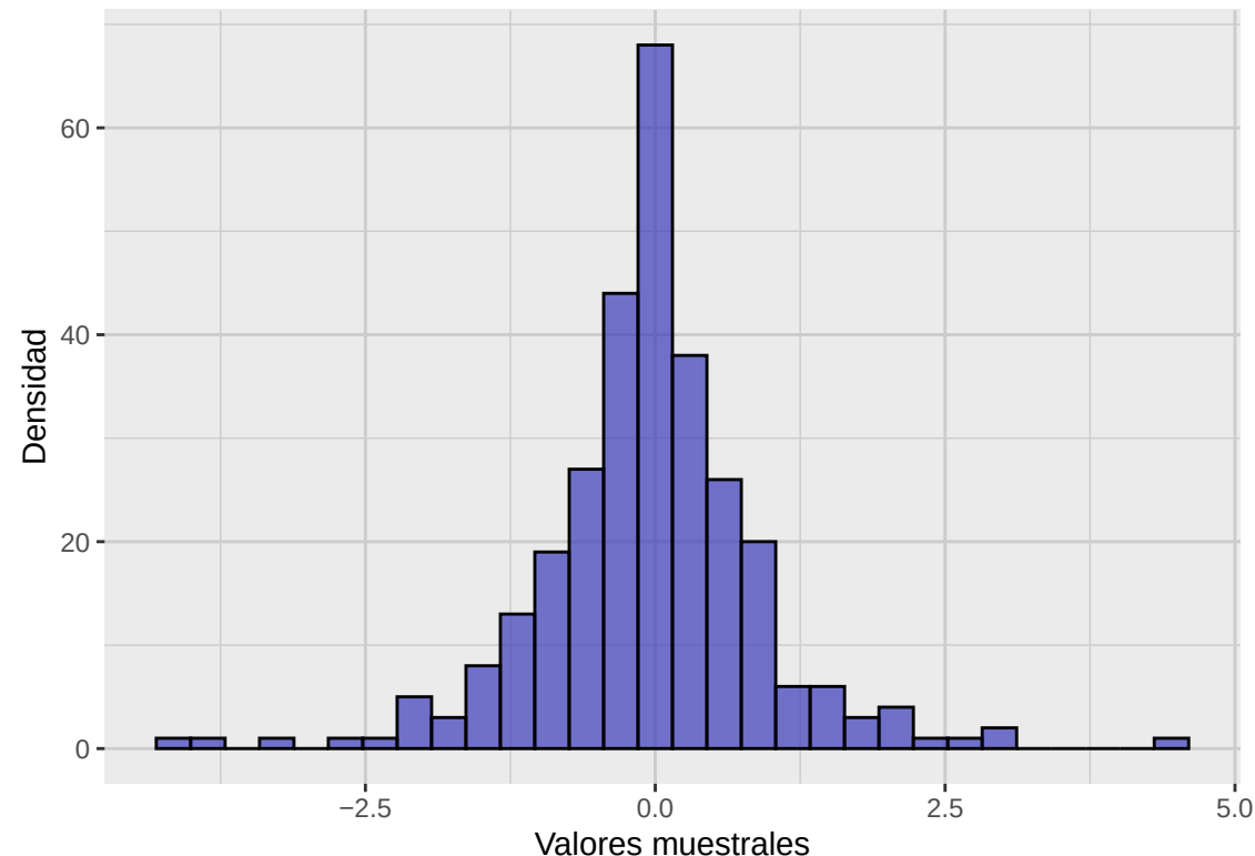
Histograma
