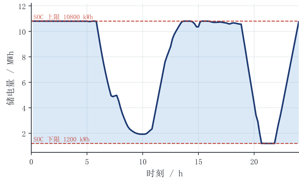
(c) 储能荷电状态的日内轨迹
