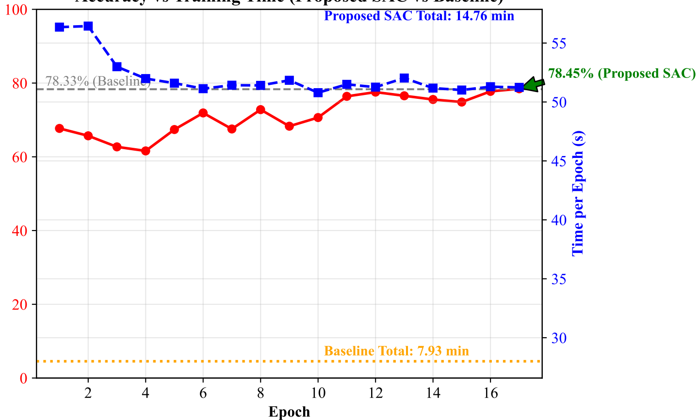
Accuracy vs Training Time (Proposed SAC vs Baseline)
