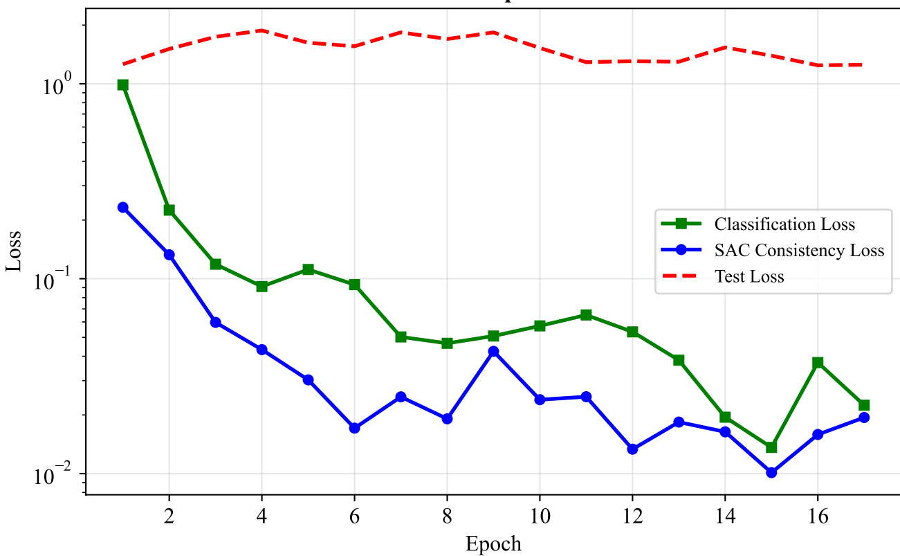
Loss Components
