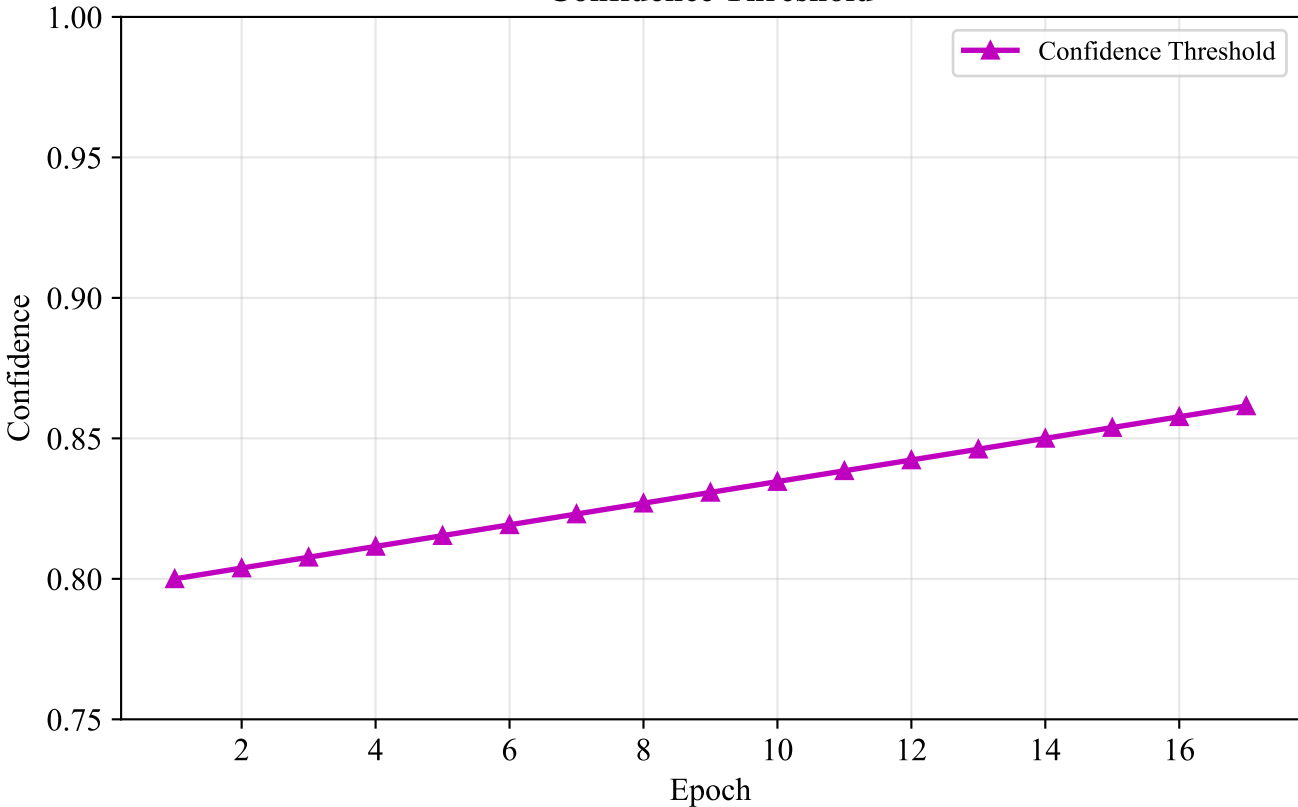
Confidence Threshold
