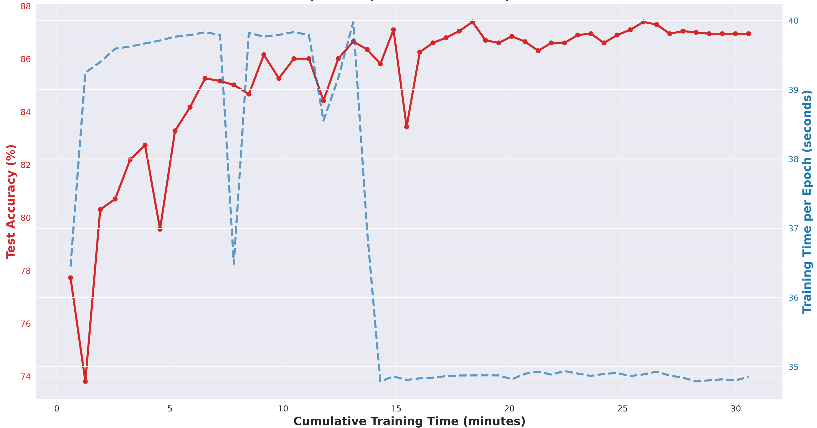
Time-Accuracy Tradeoff: MKMMD Domain Adaptation (FO → FP, Swin-T Backbone)
