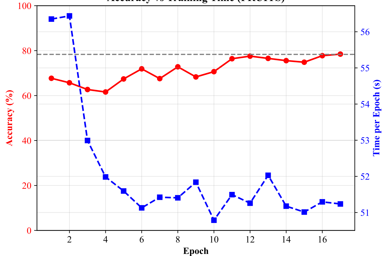
Accuracy vs Training Time (FRUITS)
