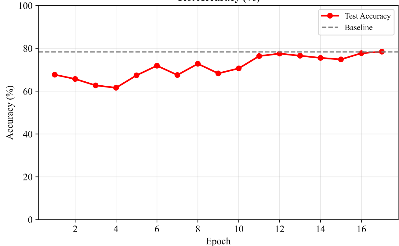
Test Accuracy (%)
