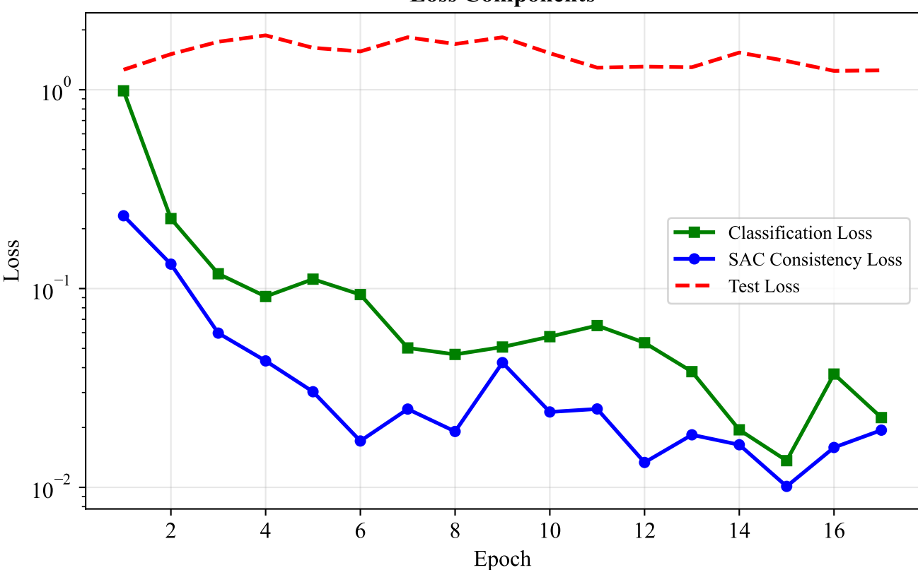
Loss Components
