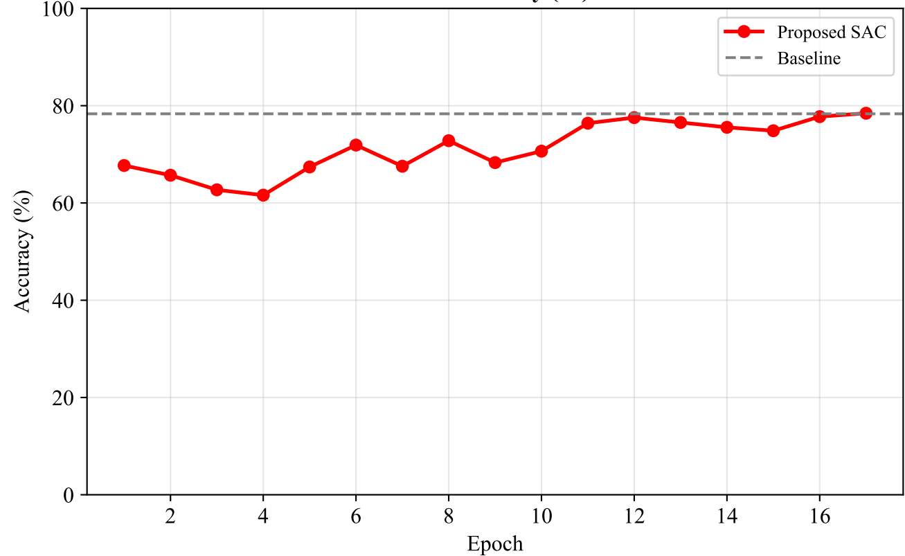
Test Accuracy (%)
