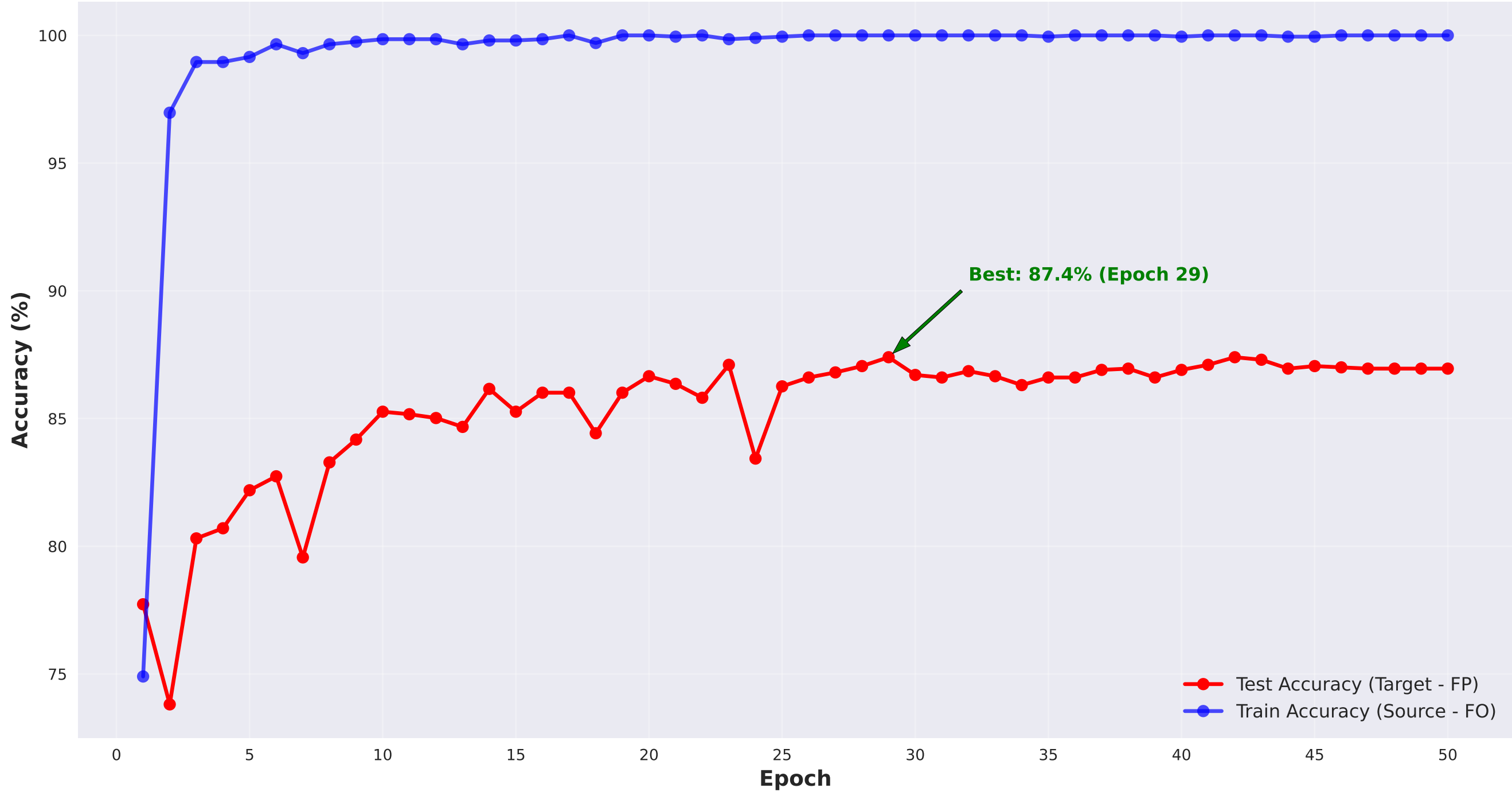
MKMMMD Performance: FO \rightarrow FP Domain Adaptation (Swin-T Backbone, 50 Epochs)
