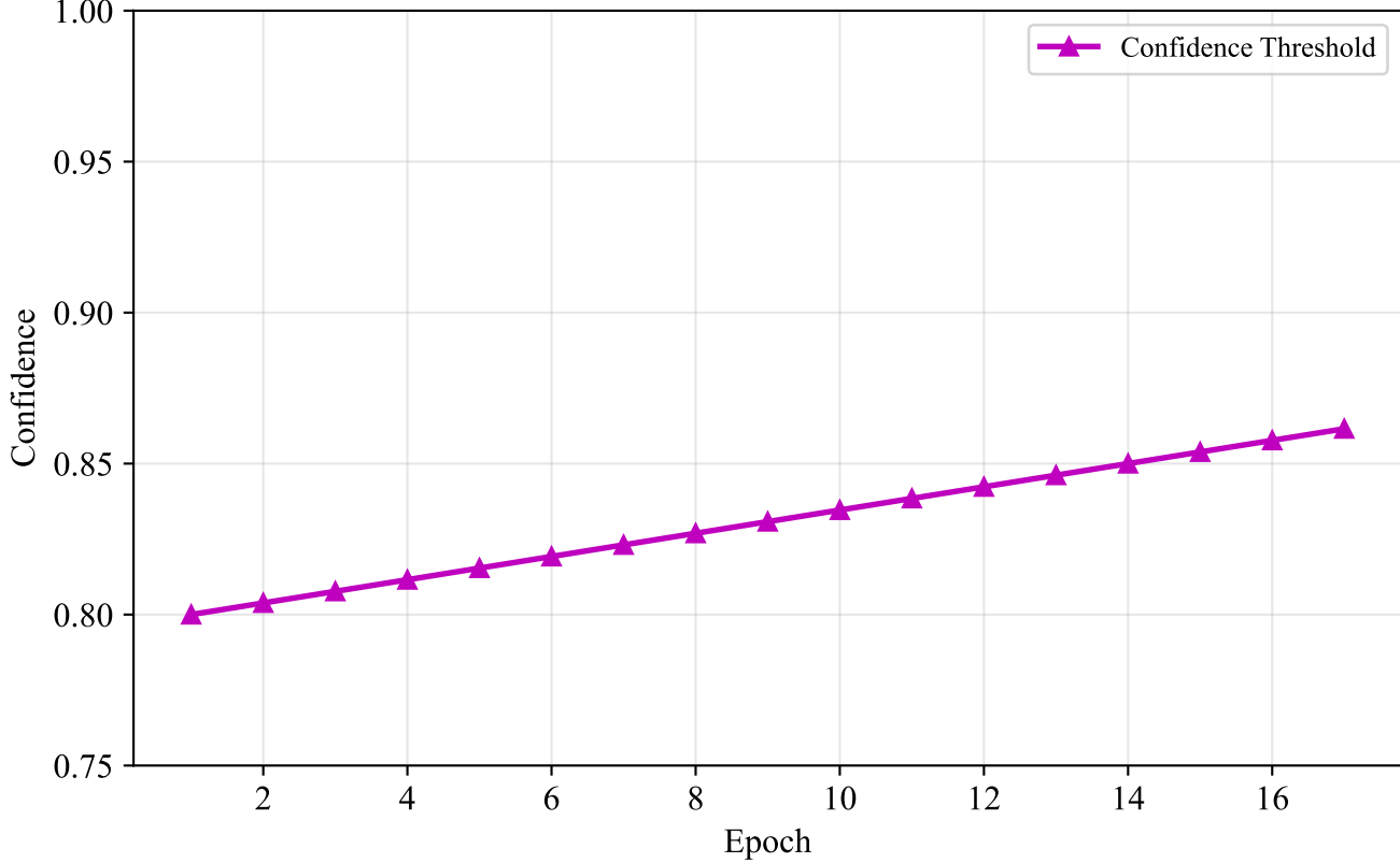
Confidence Threshold
