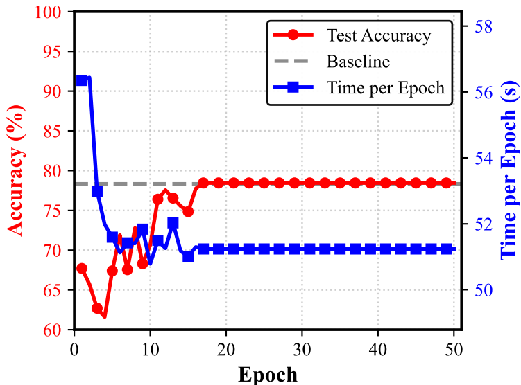
Accuracy vs Training Time (FO->FP)
