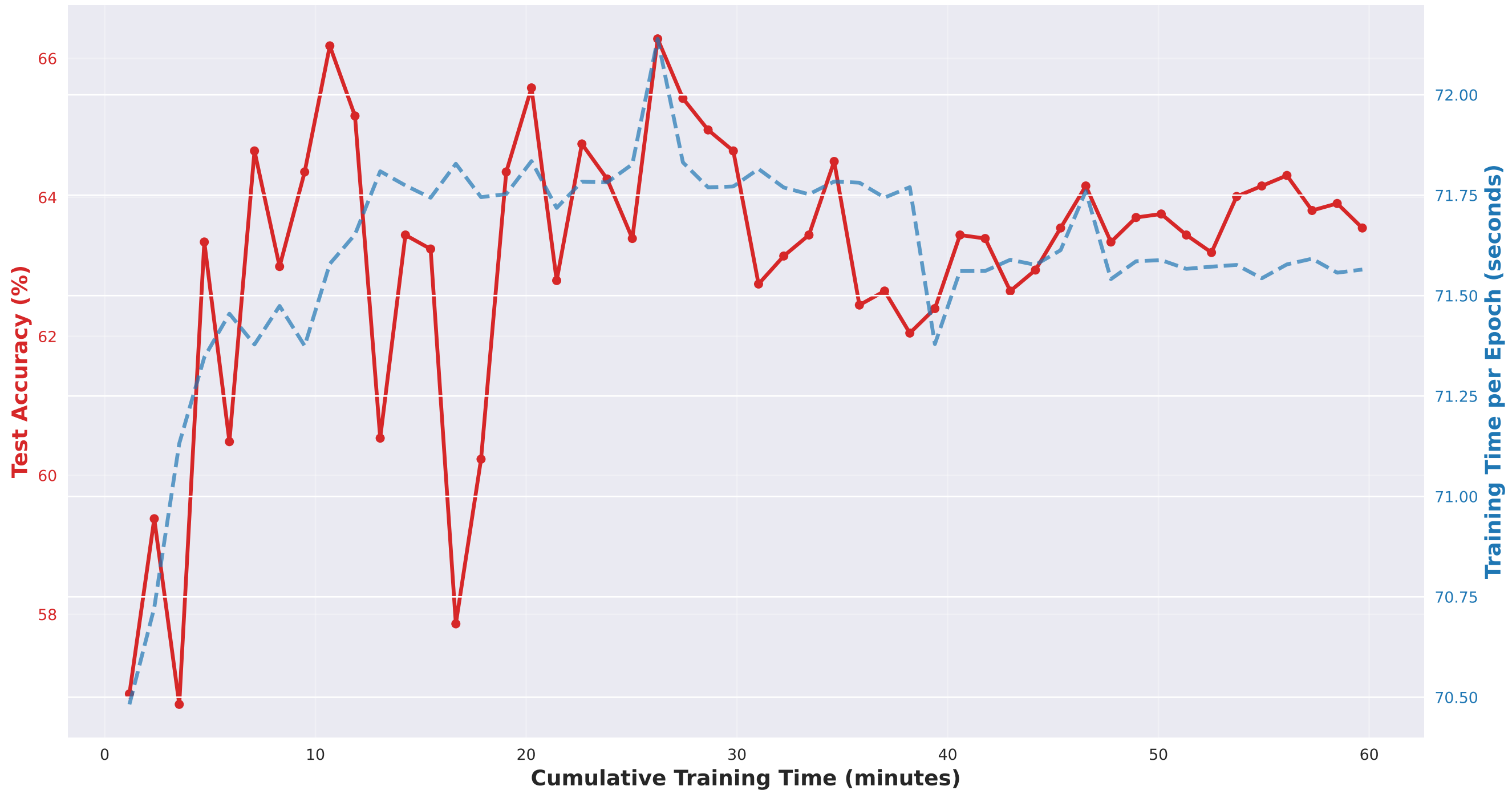
Time-Accuracy Tradeoff: SSC Domain Adaptation (FO → FP, Swin-T Backbone)
