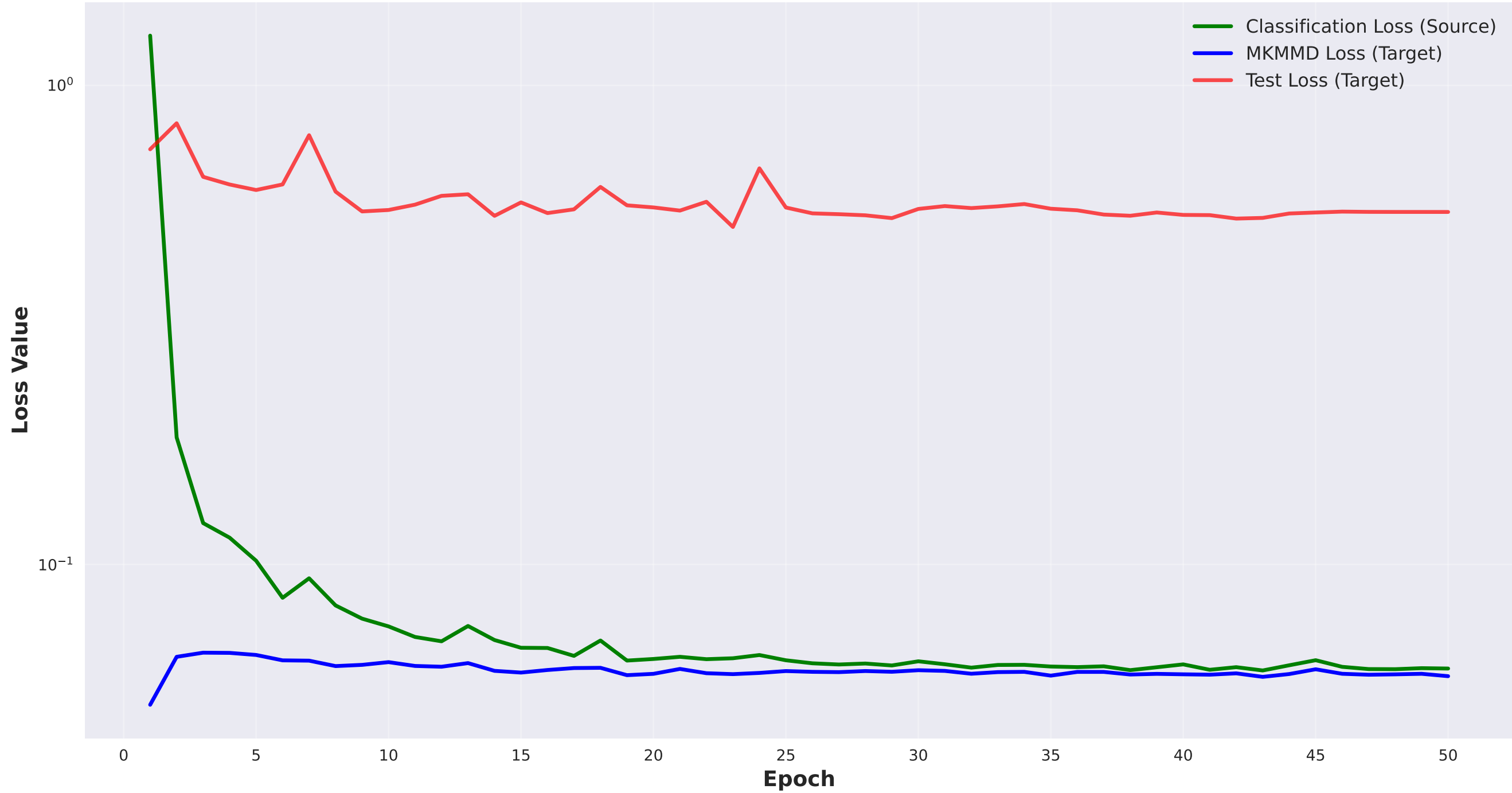
Loss Components: MKMMD Training Dynamics (FO → FP Domain Adaptation)
