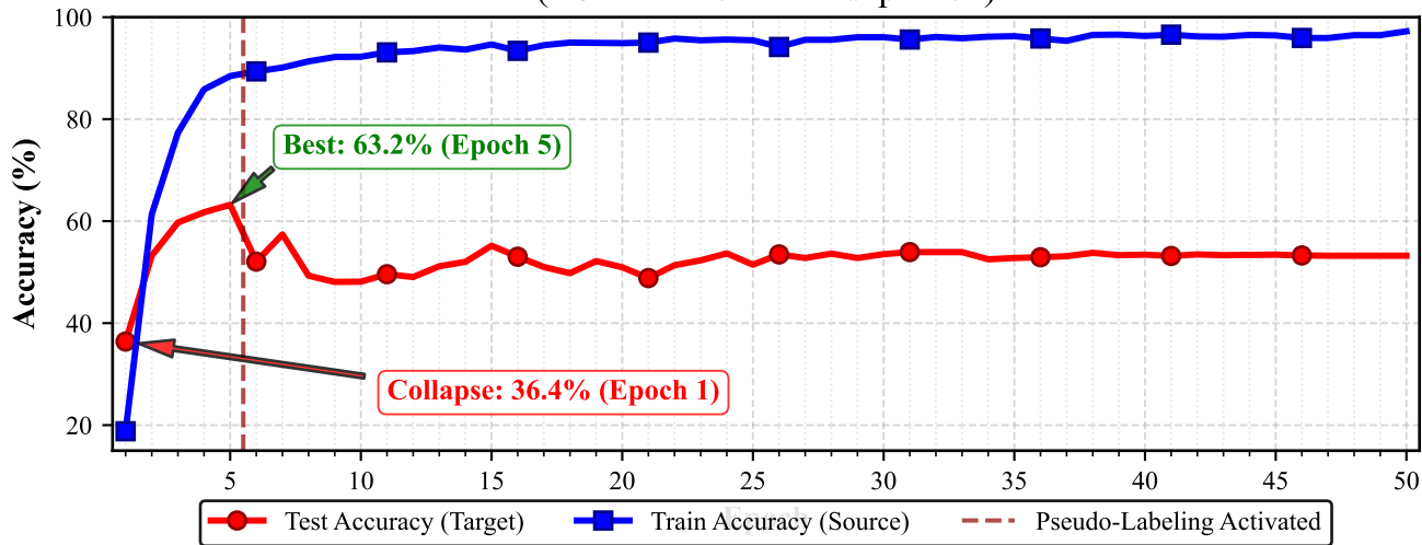
Catastrophic Collapse: SSC + Pseudo-Labeling Performance (FO \rightarrow FP Domain Adaptation)
