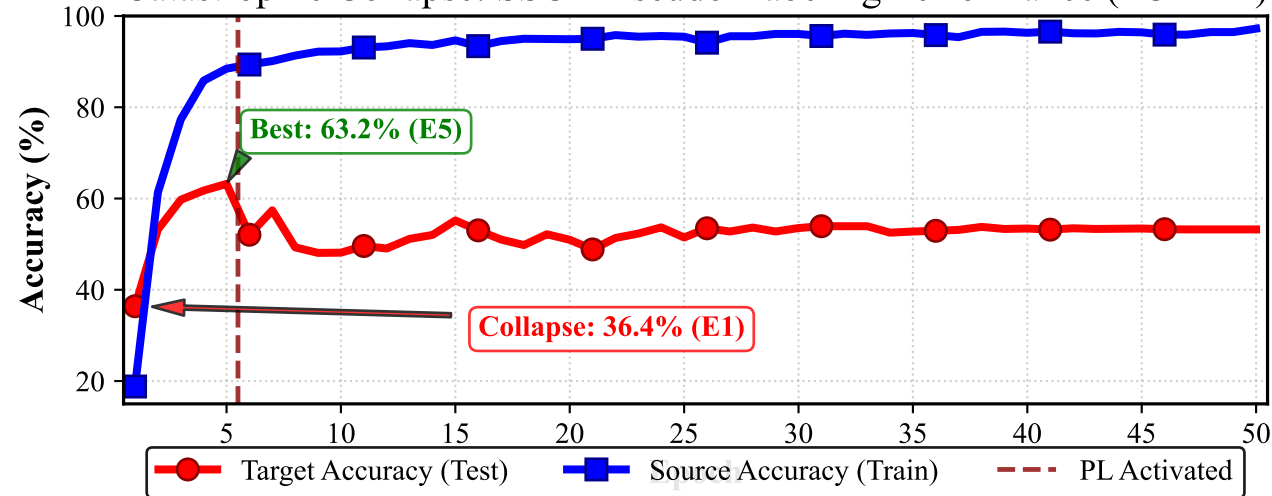
Catastrophic Collapse: SSC + Pseudo-Labeling Performance (FO \rightarrow FP)
