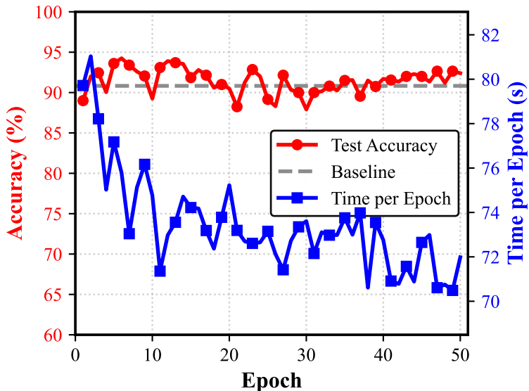
Accuracy vs Training Time (FP->FO)
