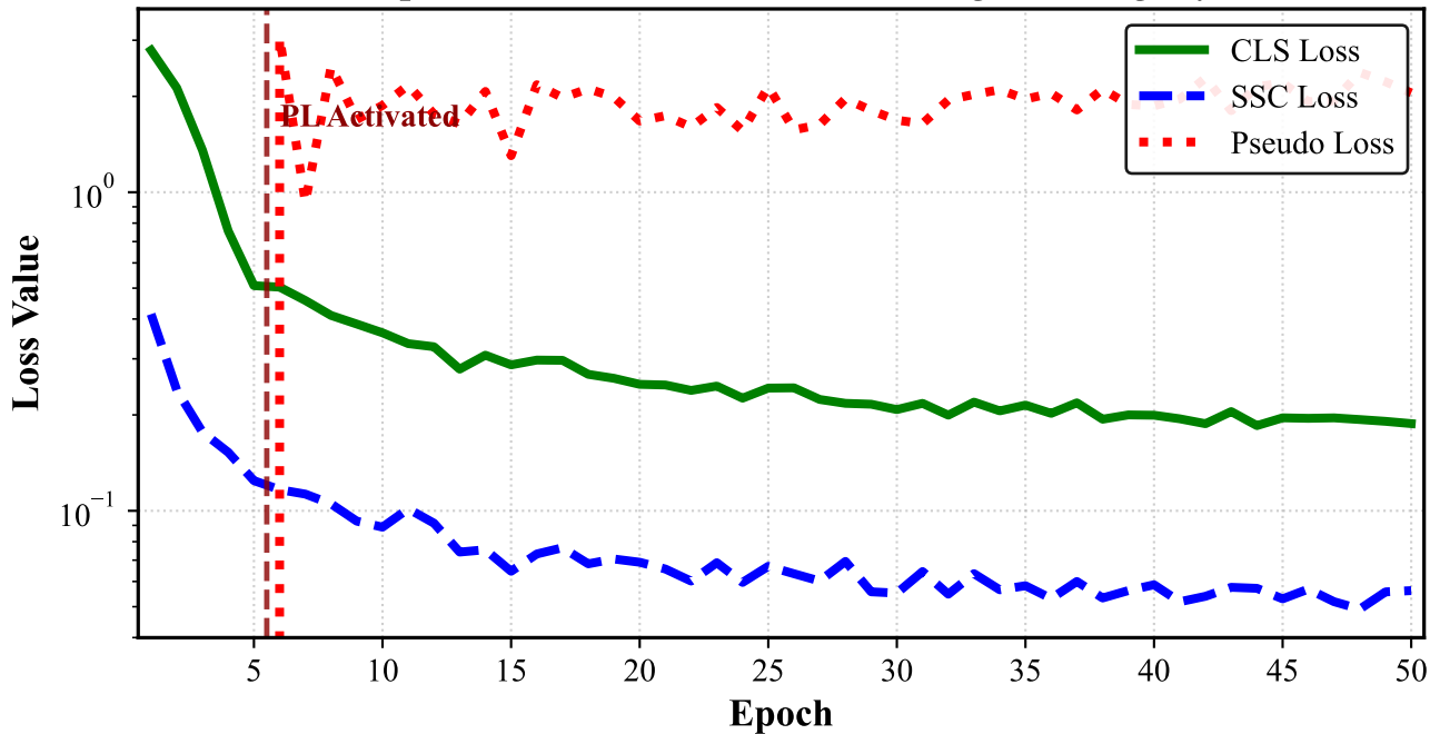
Loss Components: SSC + Pseudo-Labeling Training Dynamics
