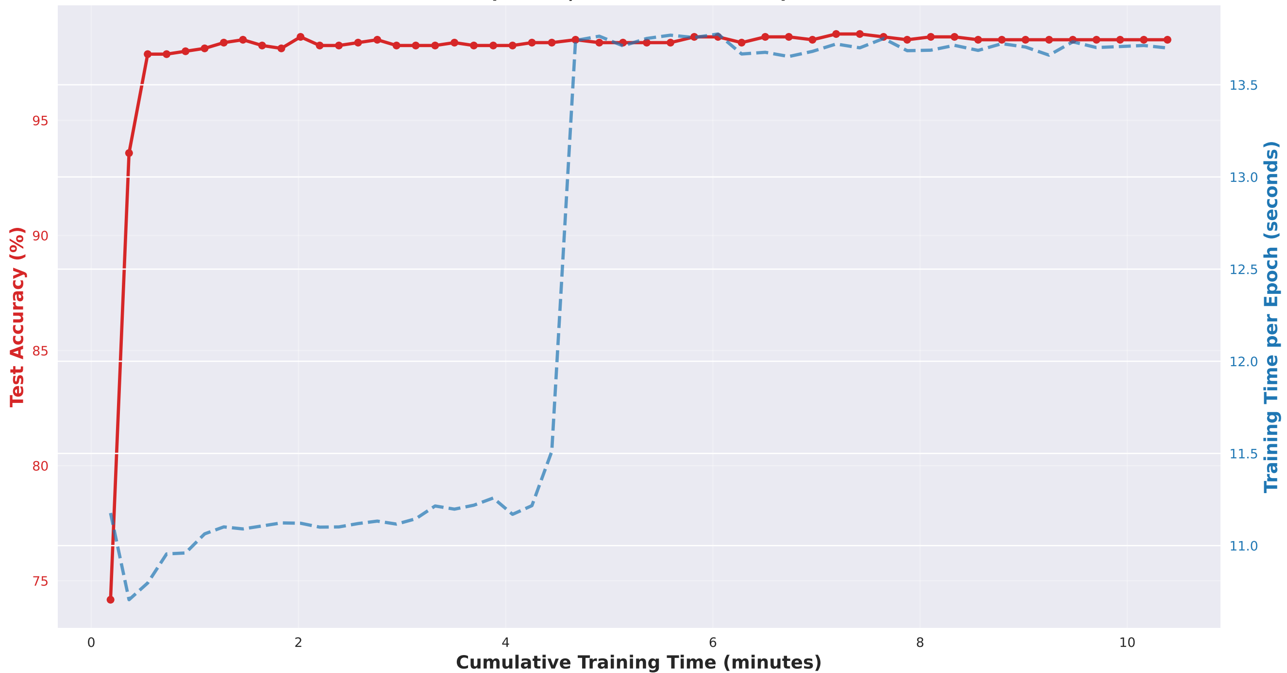
Time-Accuracy Tradeoff: MKMMD Domain Adaptation (D → W, Swin-T Backbone)
