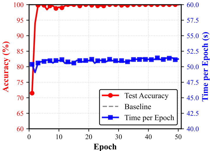
Accuracy vs Training Time (W→D)
