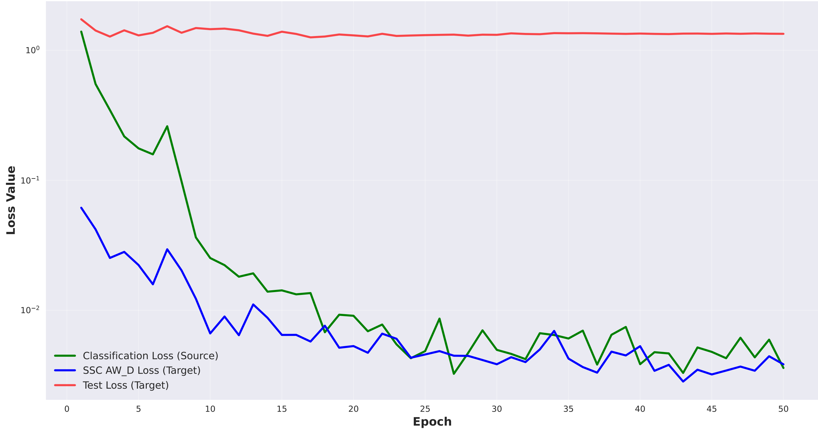
Loss Components: SSC Training Dynamics (AW → D Domain Adaptation)
