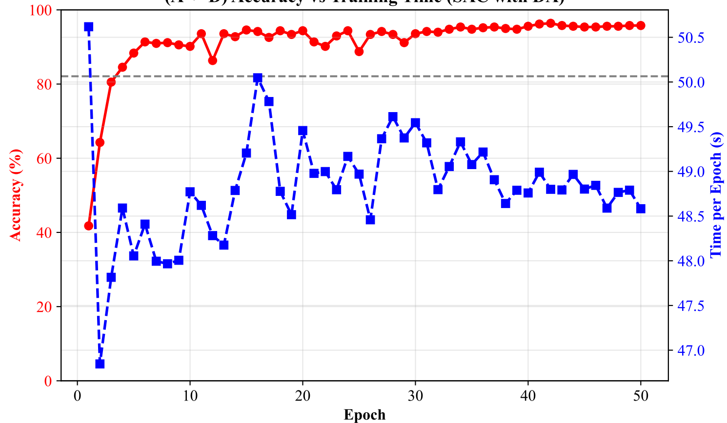
(A -> D) Accuracy vs Training Time (SAC with DA)
