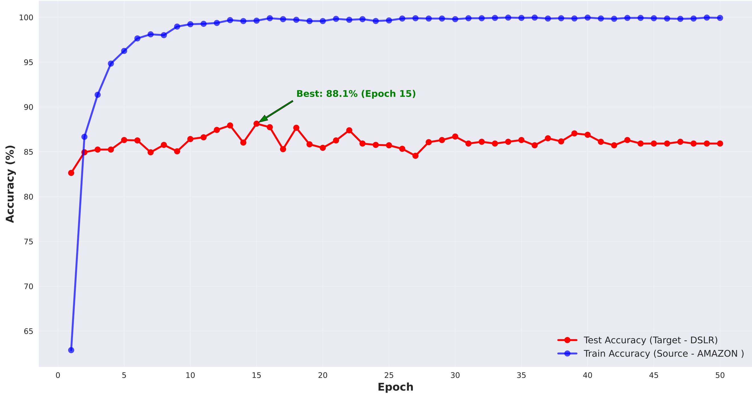
MKMMMD Performance: A \rightarrow D Domain Adaptation (Swin-T Backbone, 50 Epochs)
