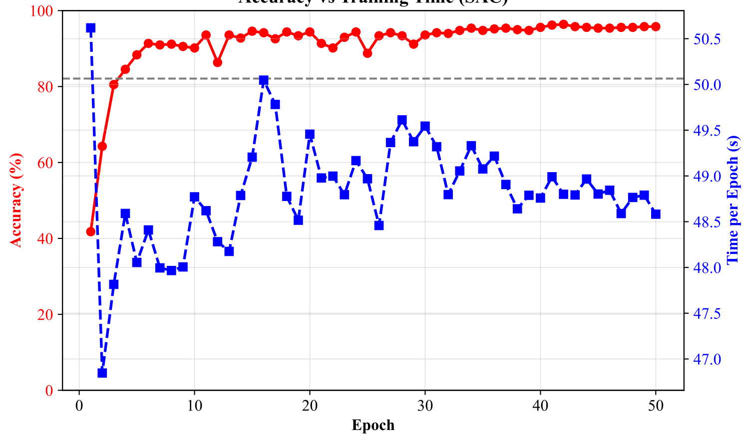
Accuracy vs Training Time (SAC)
