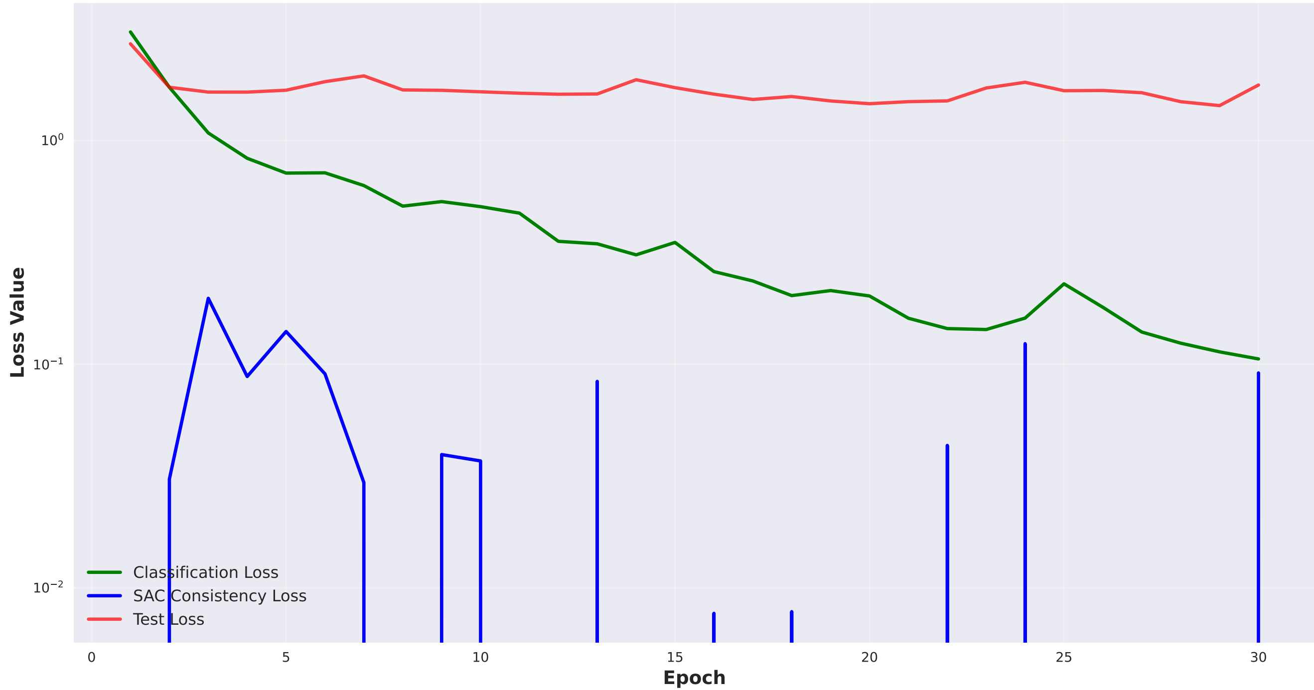
Loss Components: SAC Training Dynamics (Spectral Adversarial Consistency)
