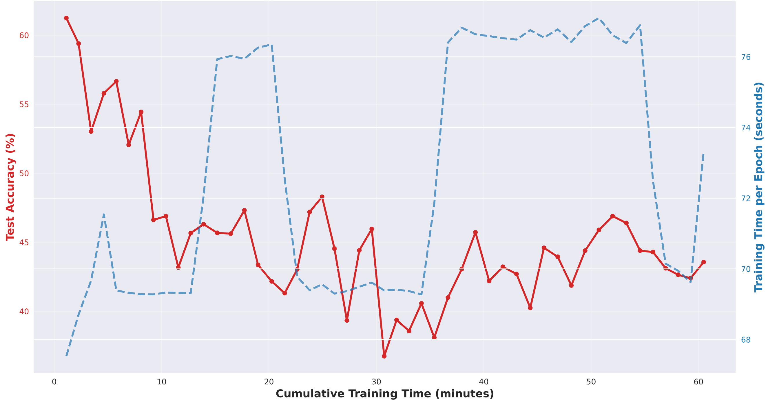
Time-Accuracy Tradeoff: SSC Domain Adaptation (AD to W, Swin-T Backbone)
