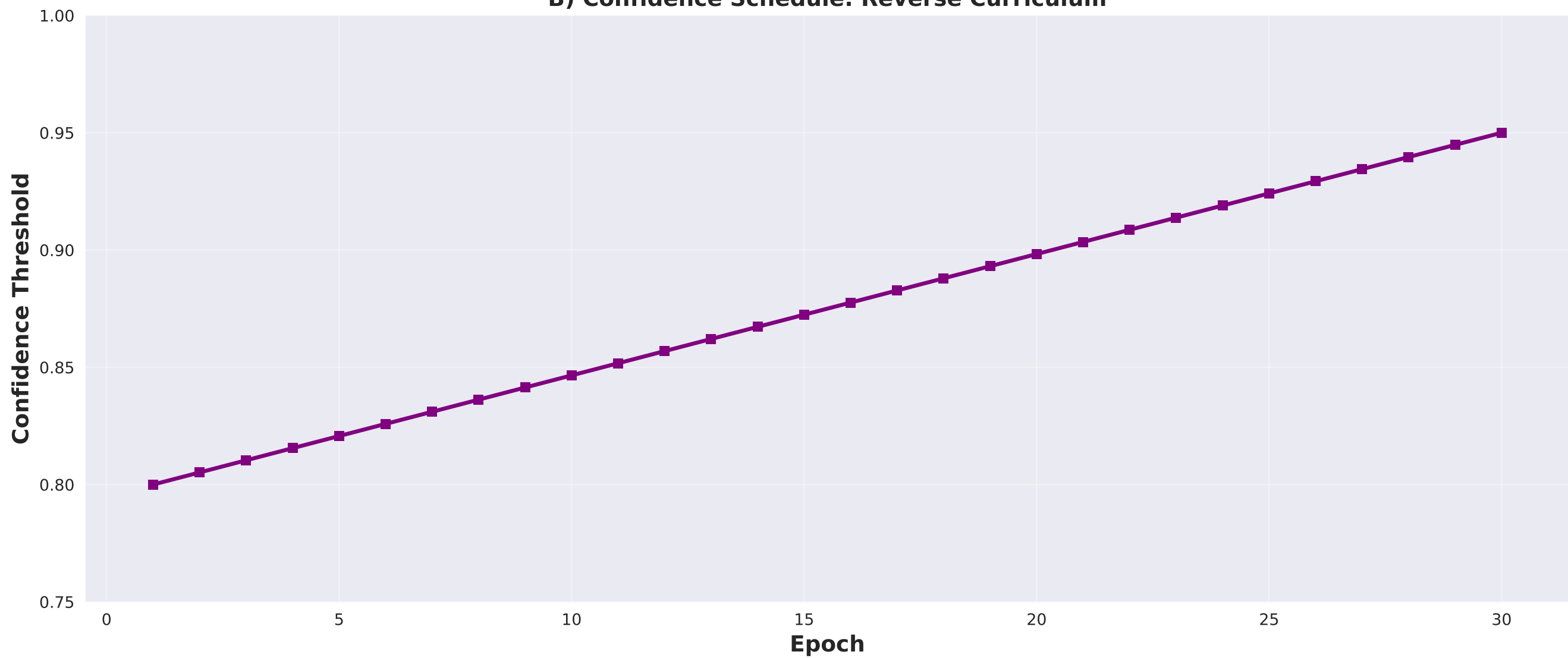
B) Confidence Schedule: Reverse Curriculum
