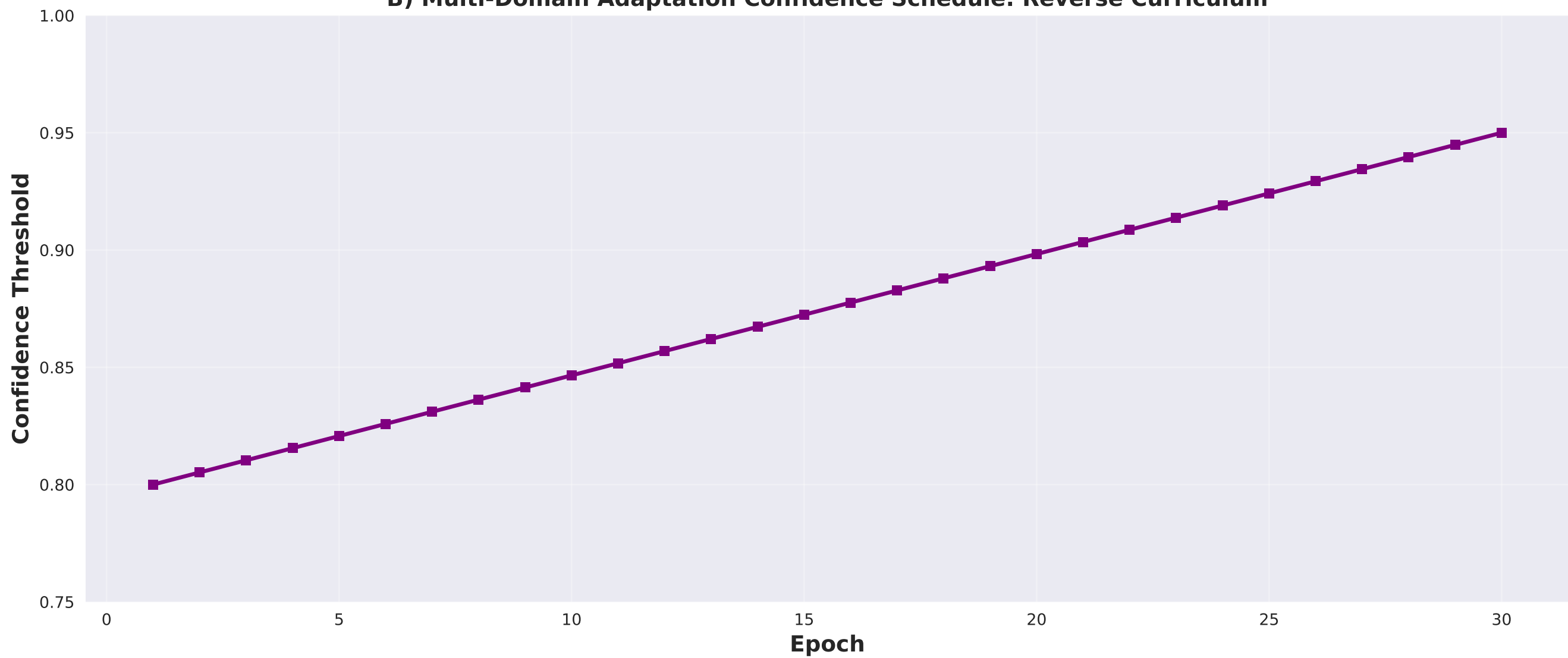
B) Multi-Domain Adaptation Confidence Schedule: Reverse Curriculum
