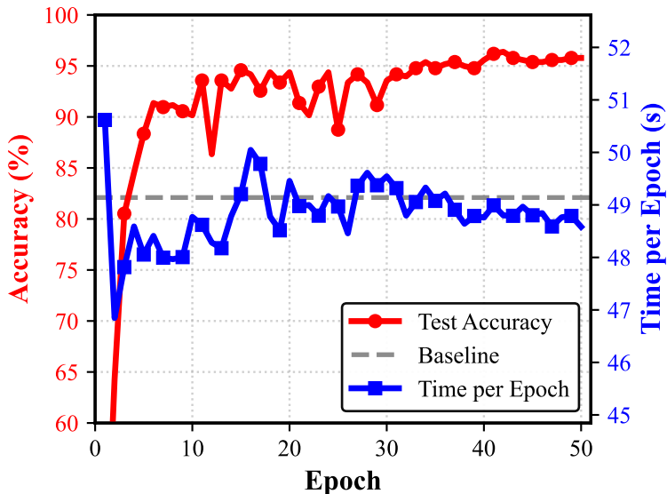
Accuracy vs Training Time (A→D)
