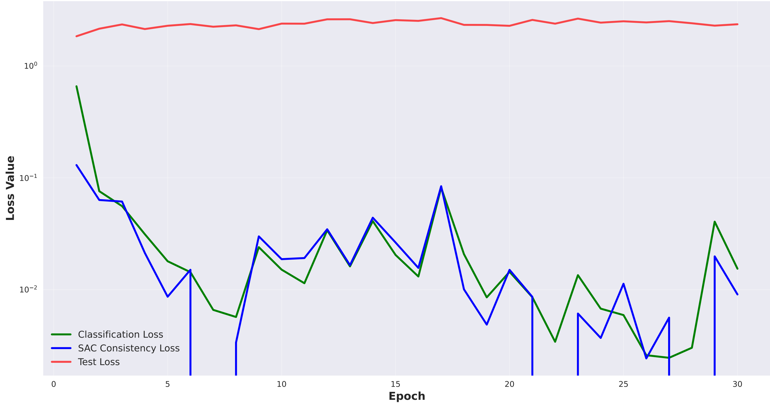
Loss Components: Multi-Domain Adaptation SAC Training Dynamics (Spectral Adversarial Consistency)
