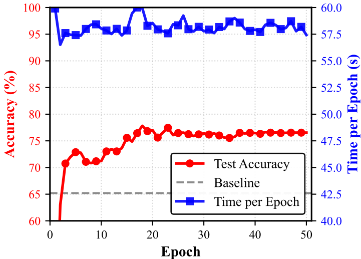
Accuracy vs Training Time (D→A)
