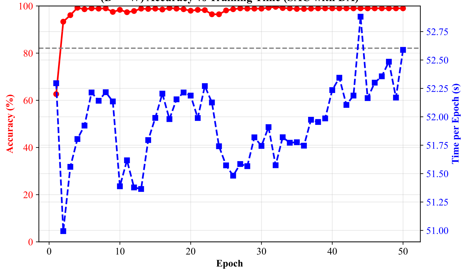
(D -> W) Accuracy vs Training Time (SAC with DA)
