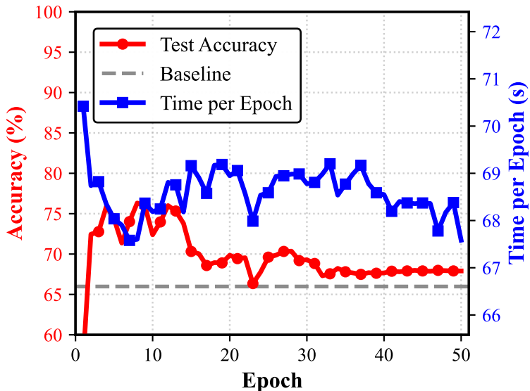
Accuracy vs Training Time (W→A)
