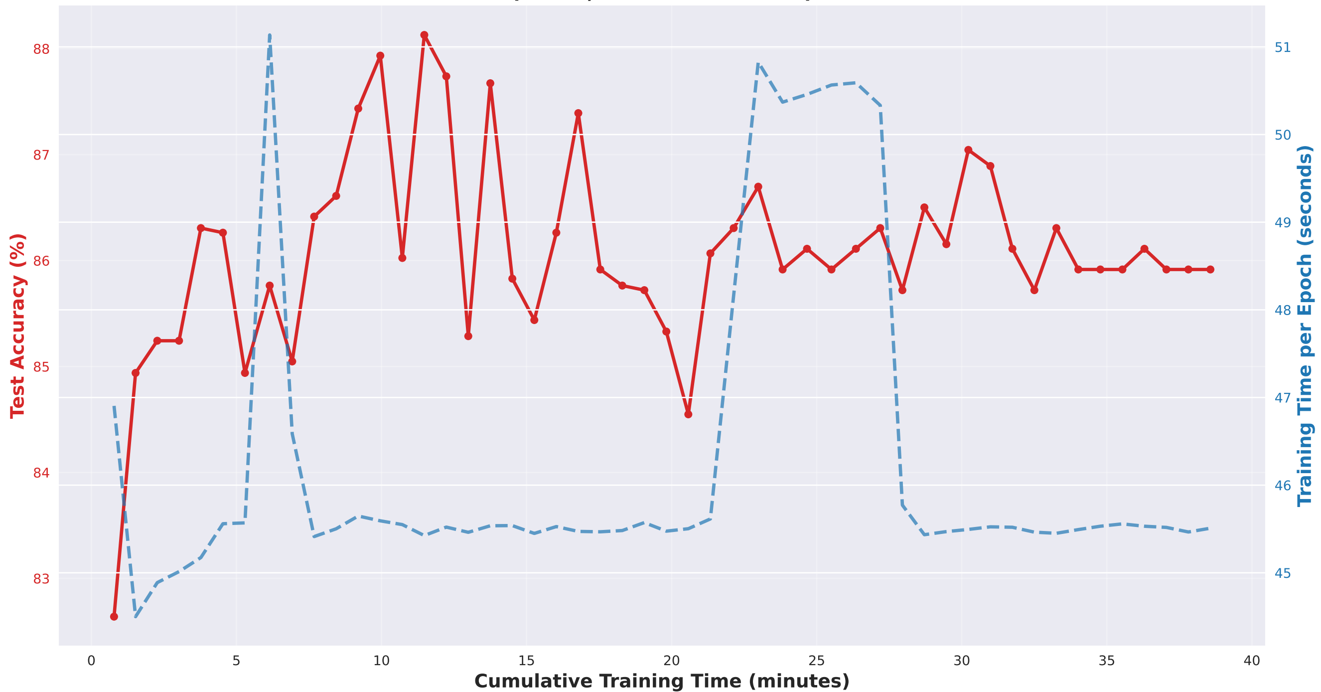
Time-Accuracy Tradeoff: MKMMD Domain Adaptation (A → D, Swin-T Backbone)
