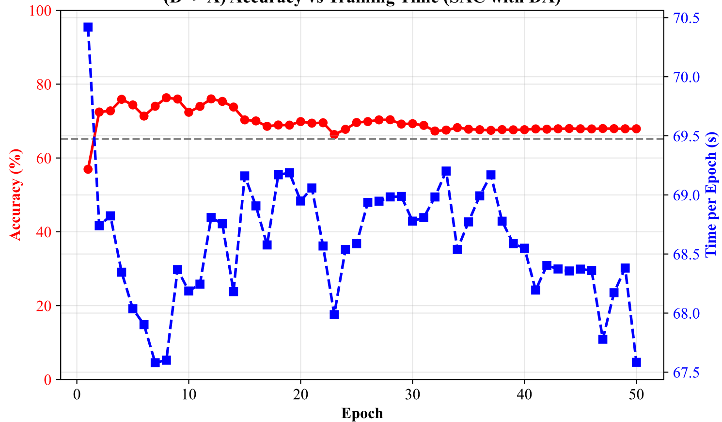
(D -> A) Accuracy vs Training Time (SAC with DA)
