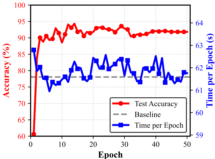
Accuracy vs Training Time (A→W)
