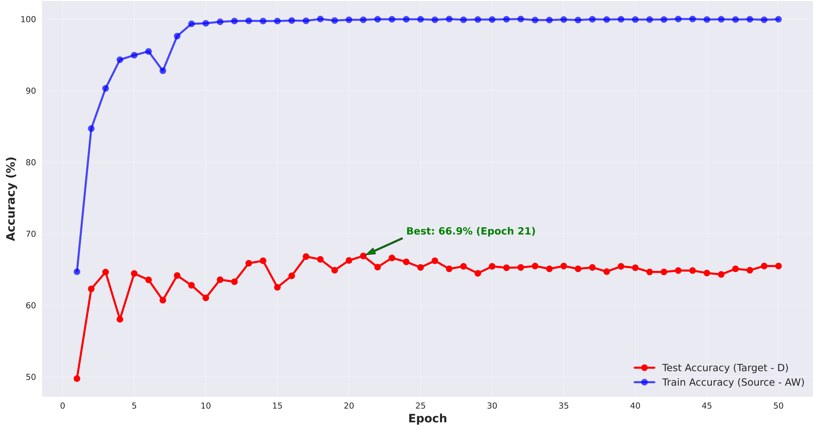
SSC Performance: AW → D Domain Adaptation (Swin-T Backbone, 50 Epochs)
