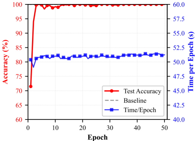
Accuracy vs Training Time (W→D)
