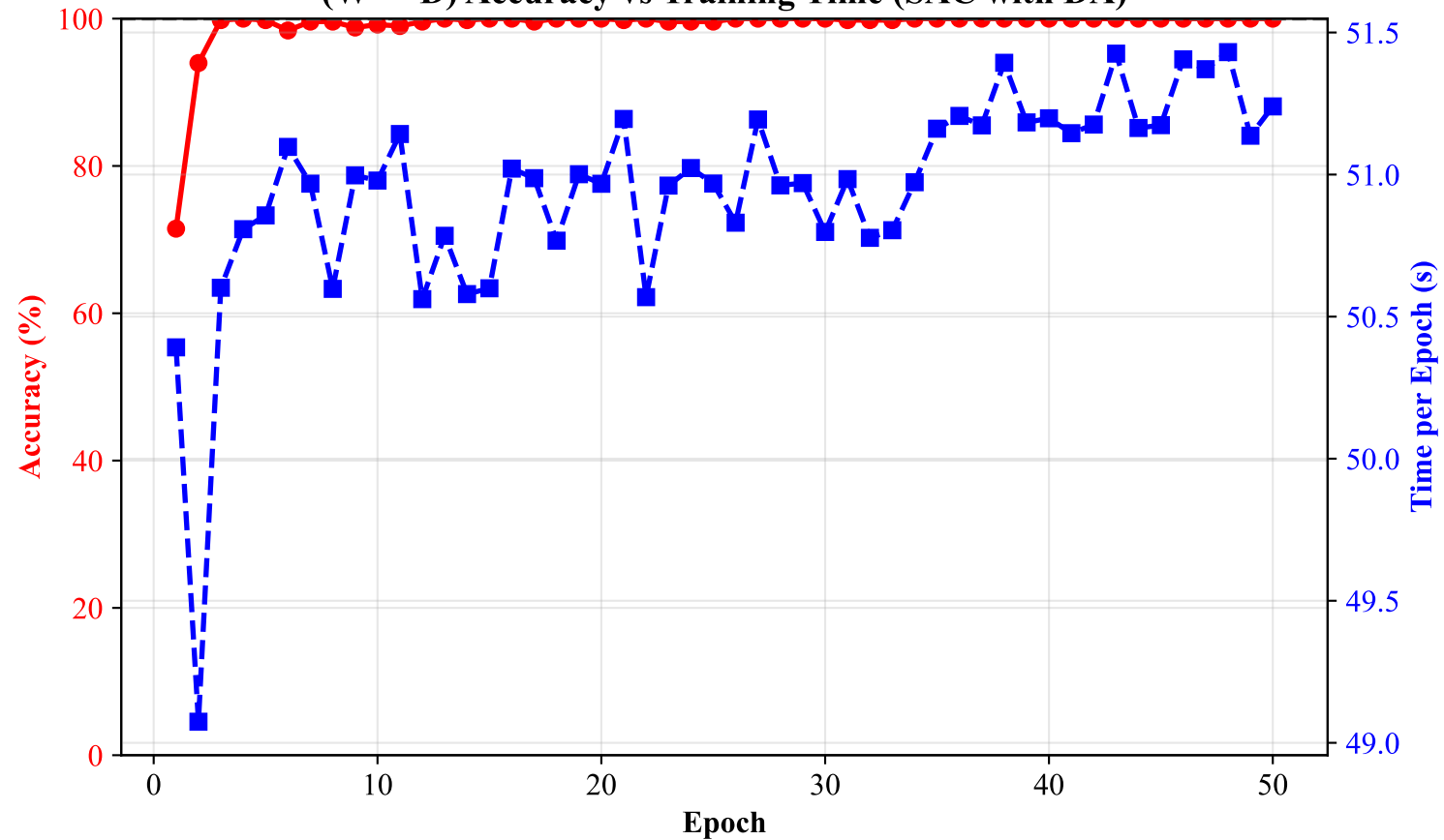
(W -> D) Accuracy vs Training Time (SAC with DA)
