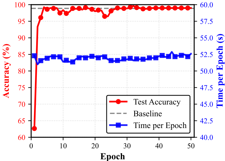
Accuracy vs Training Time (D→W)
