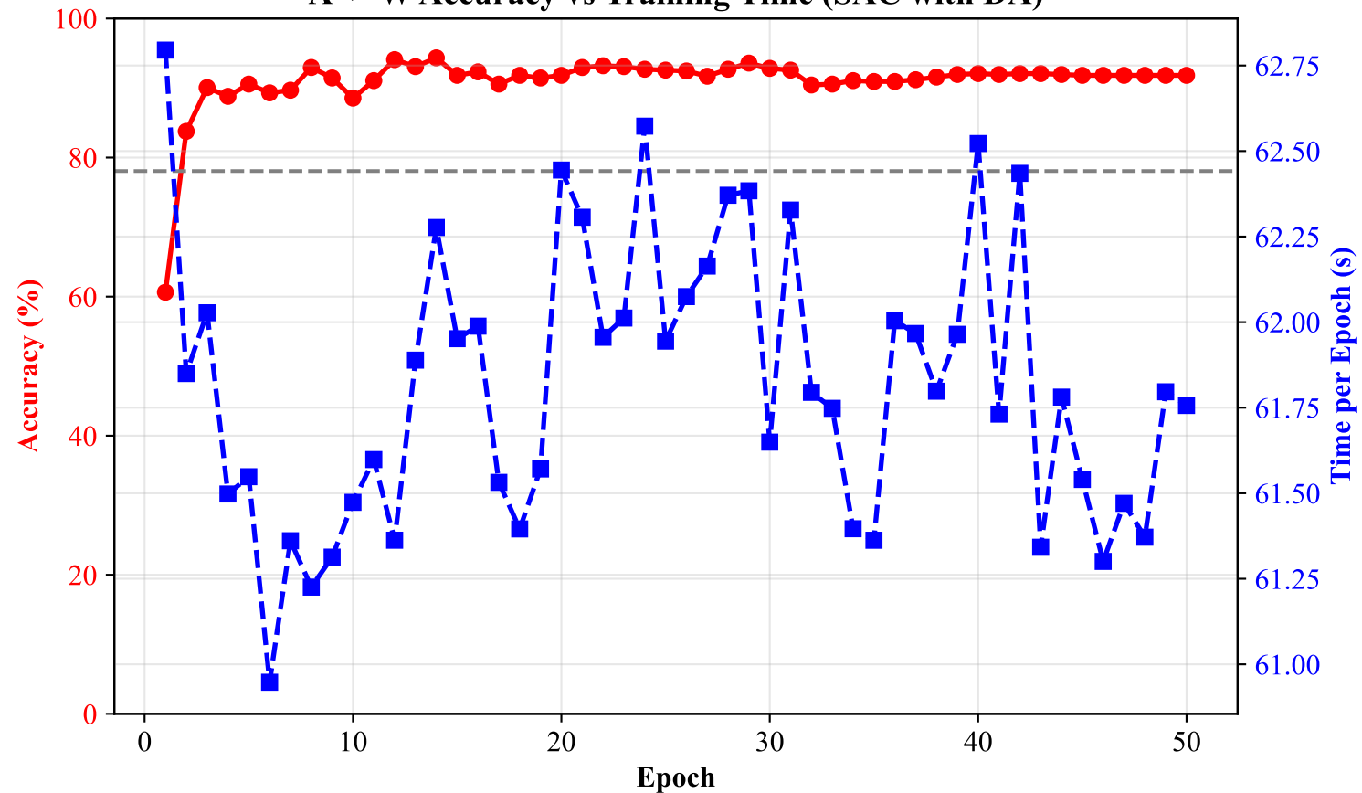
A -> W Accuracy vs Training Time (SAC with DA)
