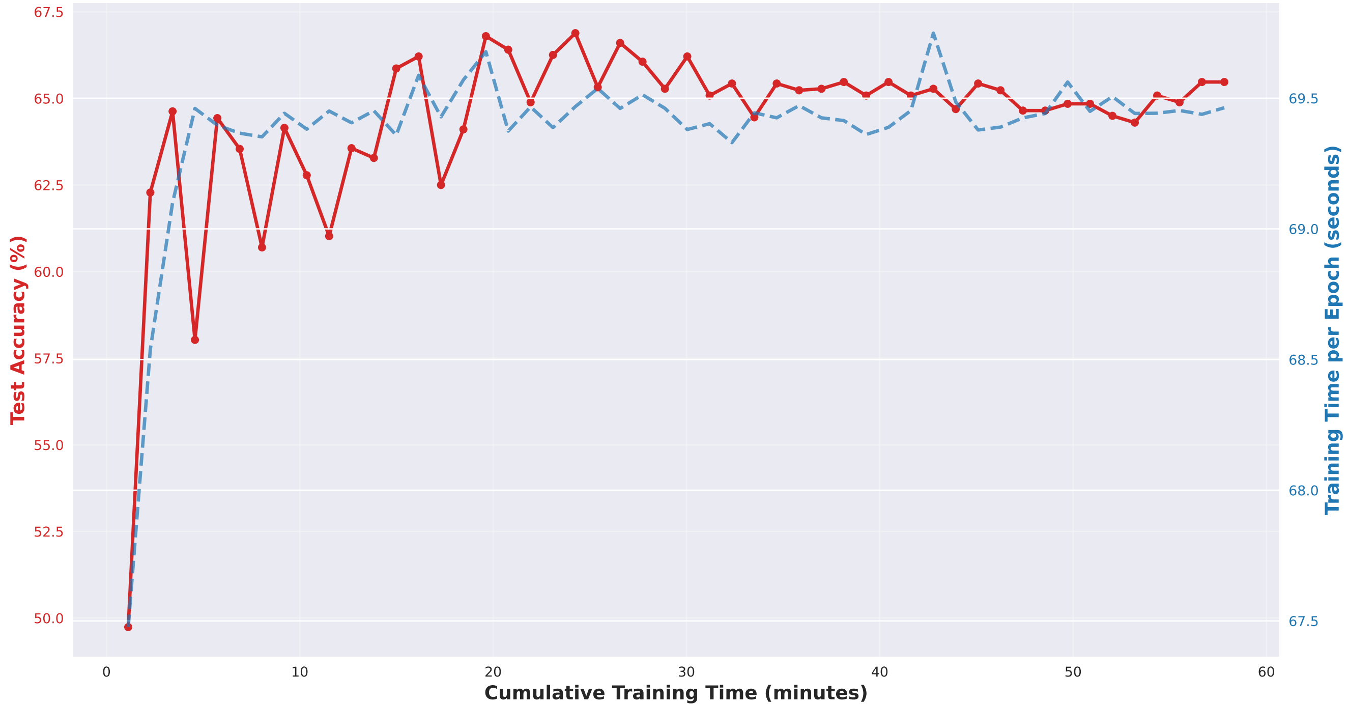
Time-Accuracy Tradeoff: SSC Domain Adaptation (Aw to d, Swin-T Backbone)
