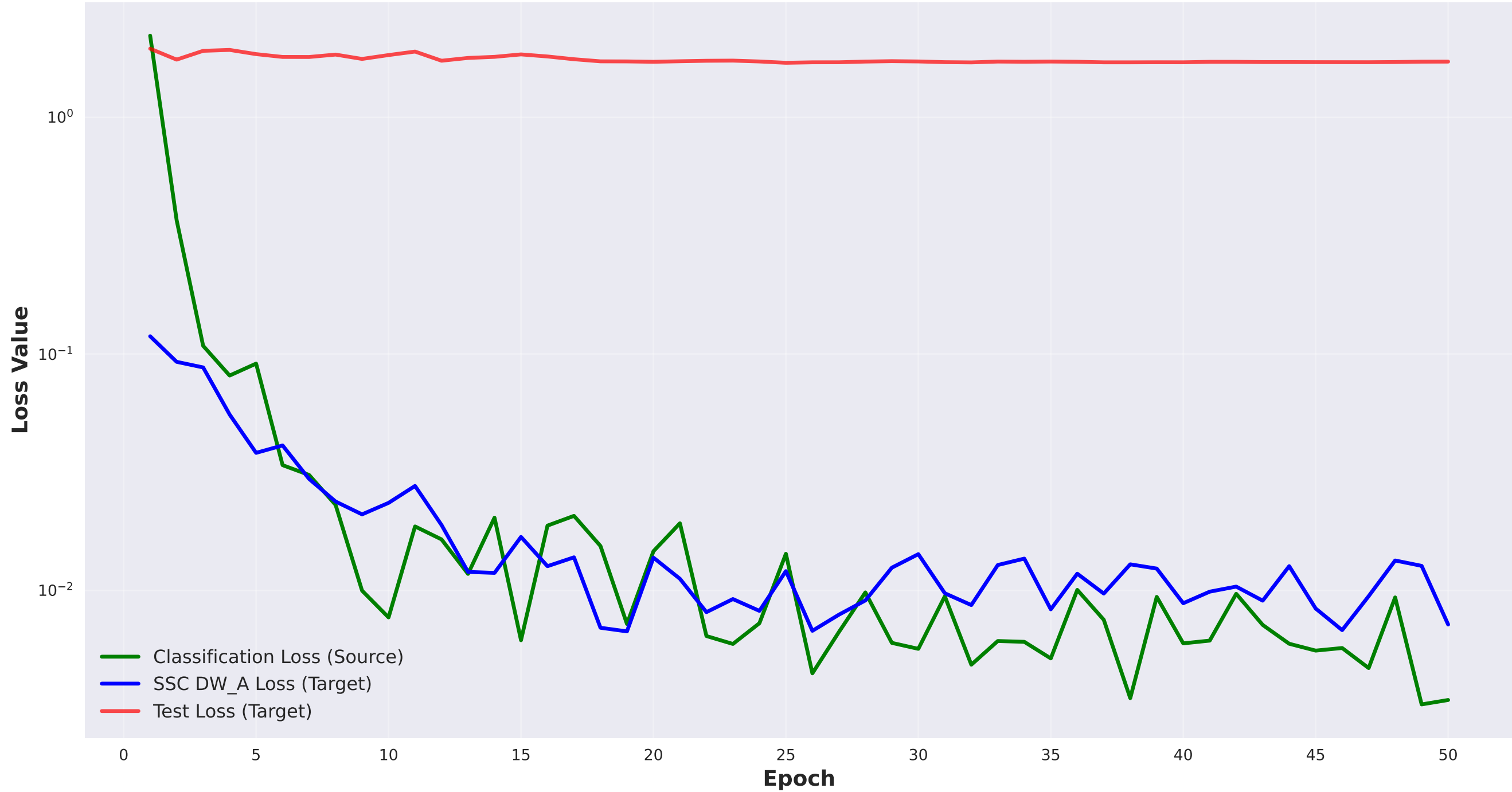
Loss Components: SSC Training Dynamics (DW → A Domain Adaptation)
