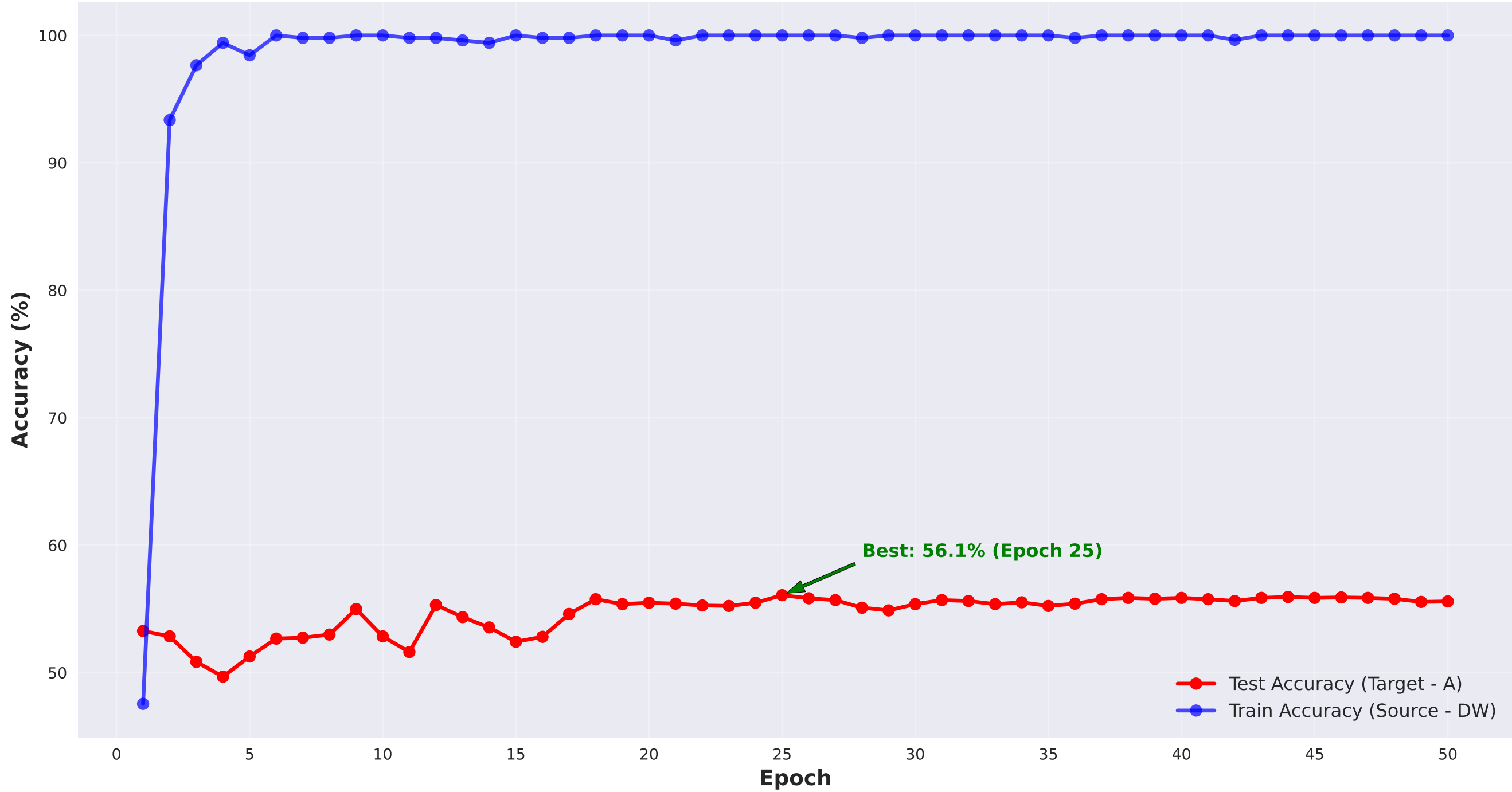
SSC Performance: DW → A Domain Adaptation (Swin-T Backbone, 50 Epochs)
