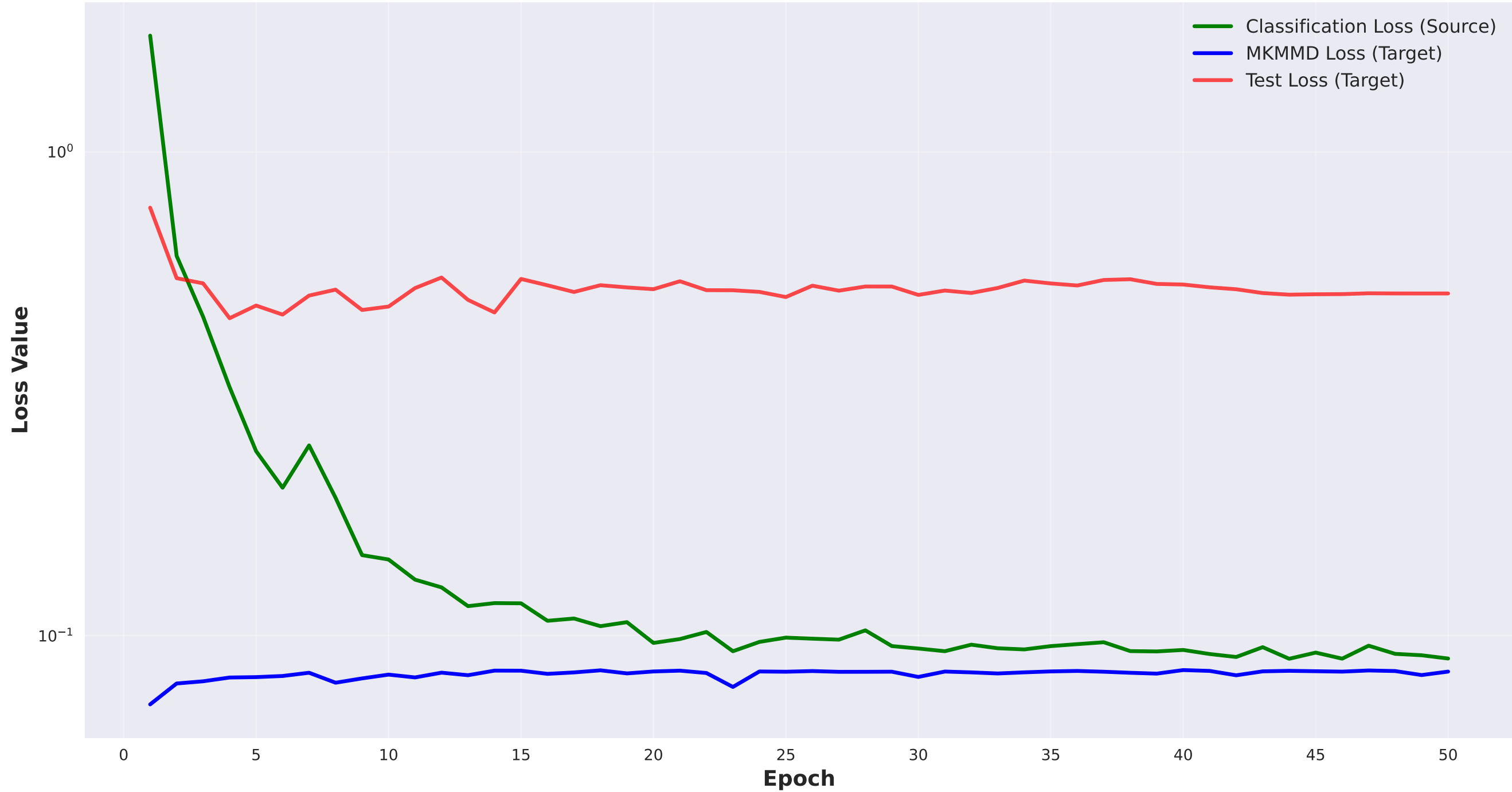
Loss Components: MKMMD Training Dynamics (A \rightarrow W Domain Adaptation)
