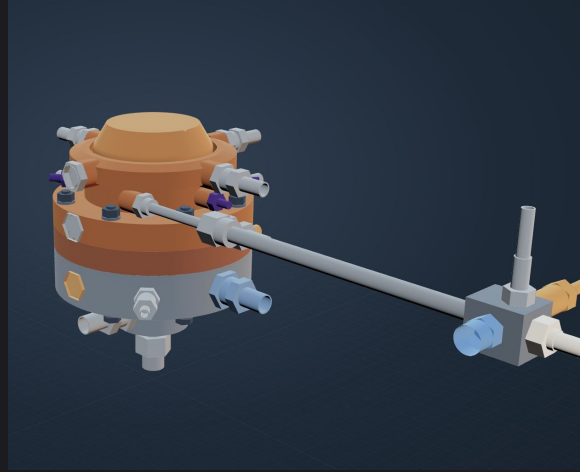
Full Injector & Chamber Assembly
