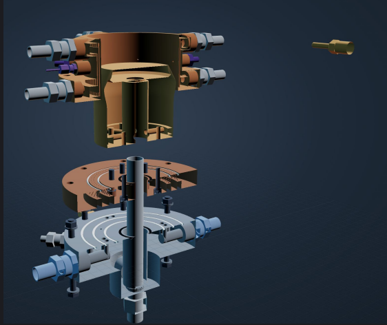
Resonance Gen-1 engine internal CAD
