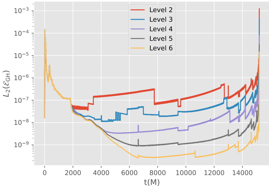
L_2(\mathcal{E}_{\text{GH}}) vs t(\text{M}) for Sim09
