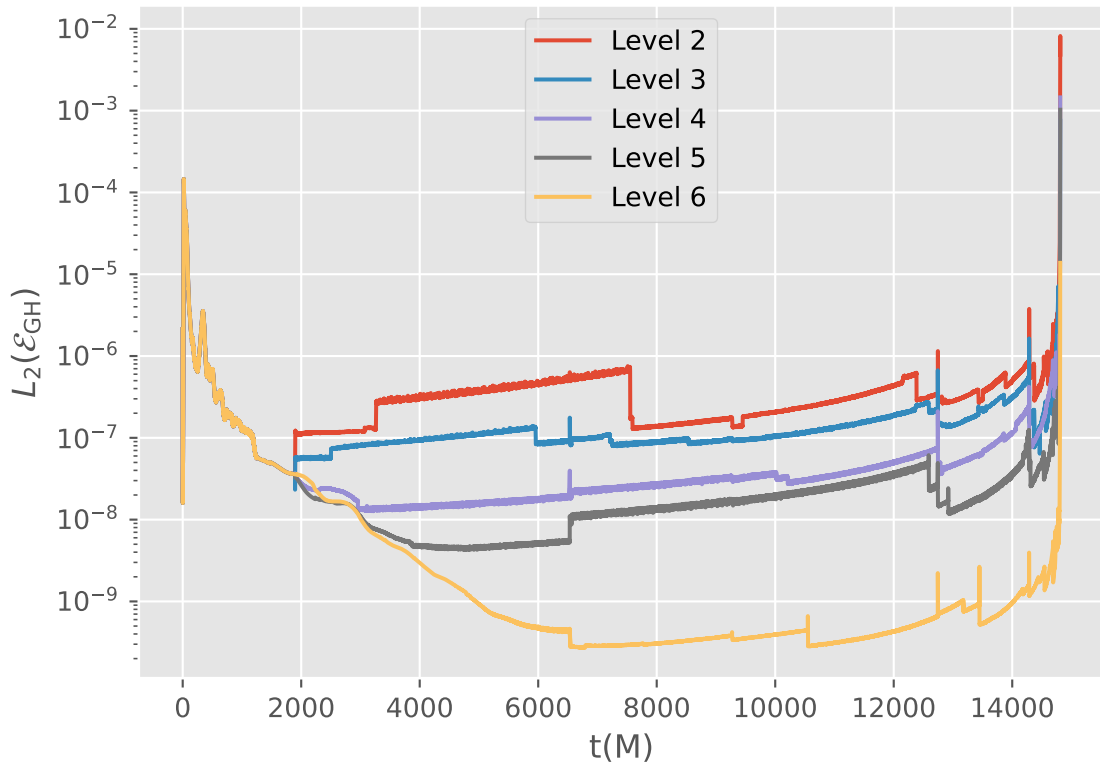
L_2(\mathcal{E}_{GH}) vs t(M) for Sim11
