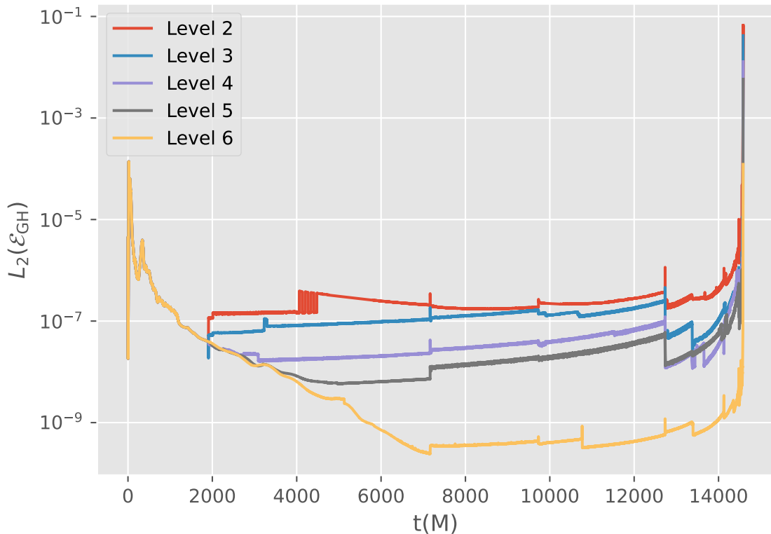
L_2(\mathcal{E}_{GH}) vs t(M) for Sim12
