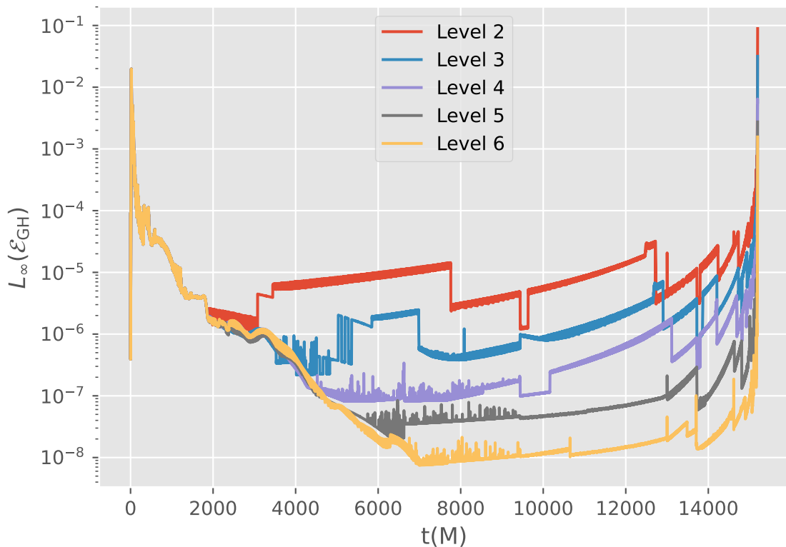
L_\infty(\mathcal{E}_{\text{GH}}) vs t(\text{M}) for Sim09
