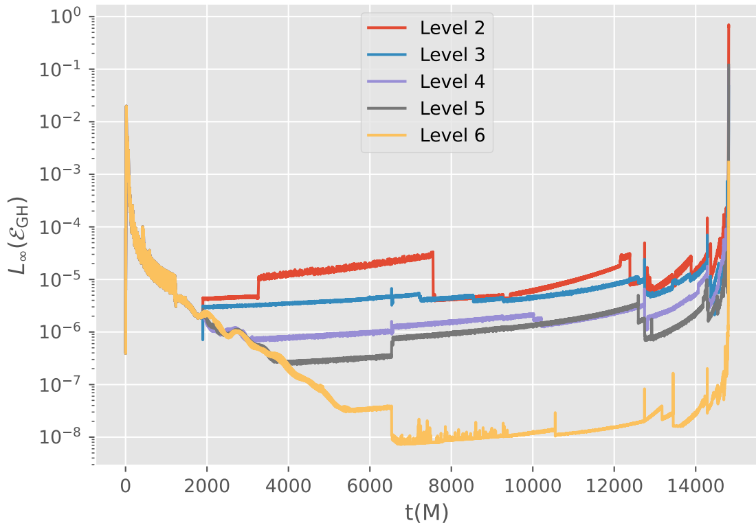
L_\infty(\mathcal{E}_{\text{GH}}) vs t(\text{M}) for Sim11
